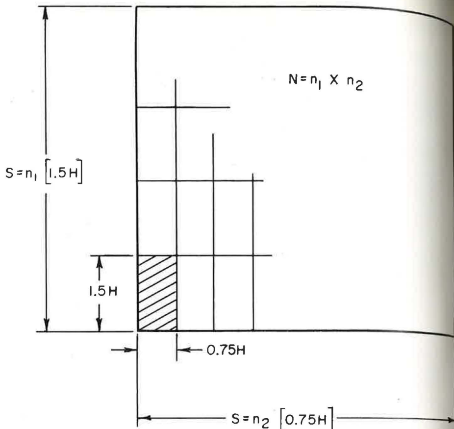
FIGURE A-1
