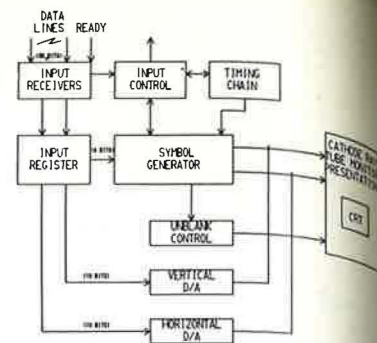
BASIC dd 40 BLOCK DIAGRAM
