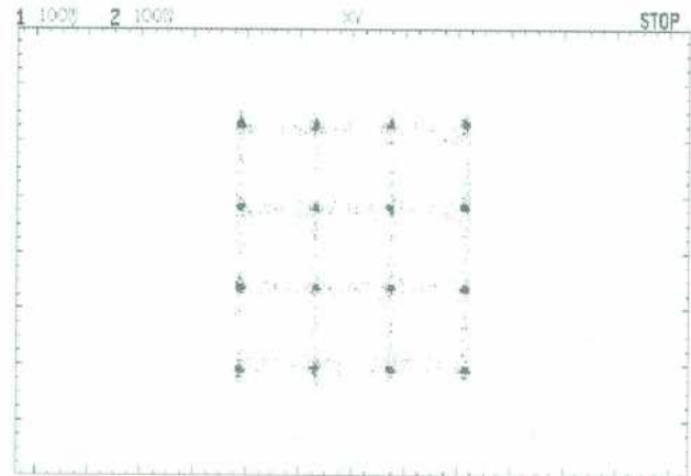
Fig. 9. A 16-QAM constellation plot from an HP 54600A oscilloscope, captured using the I-Q option of the HP 71910A.
