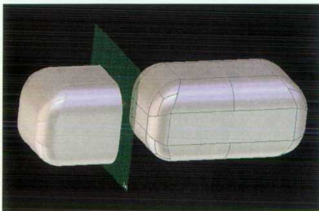
Fig. 12. A body with a green reflection plane set up and, at right, the result of the reflect operation.
