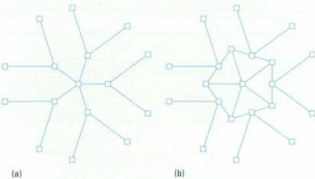
Fig. 16. (a) Topology of a vertex region where five faces meet after extending the edges. (b) Topology created for the representation of the vertex region.
