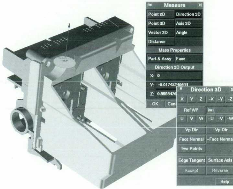
Fig. 5. When the user has to enter a value for a command, the system provides the appropriate tools for data entry. The result is displayed either textually or graphically as part of the model.
