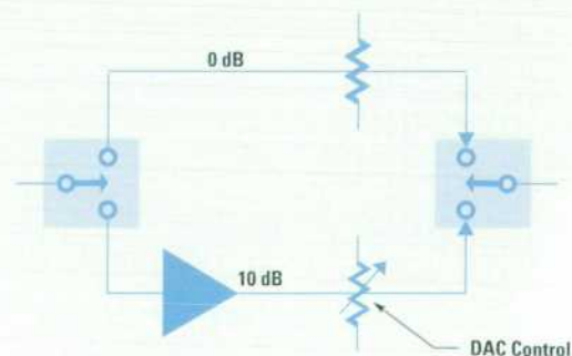
Fig. 15. A block diagram of the step gains in the HP 70911A.
