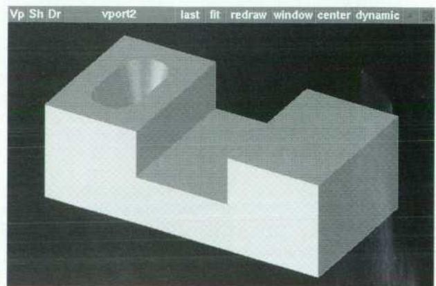
Fig. 2. Another example of the limitations of LOPs. The pocket in the left top face cannot be copied or moved to the right top face using LOPs because both top faces would change topology by adding or removing faces and edges.
