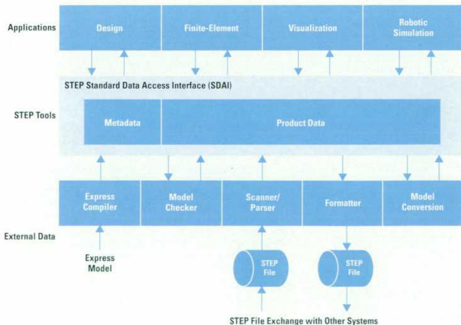
Fig. 13. PRODEX STEP tools architecture.
