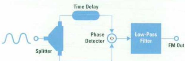
Fig. 23. Time-delay discriminator.
