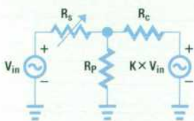
Fig. 4. Topology for a feed-forward amplitude compensation circuit.
