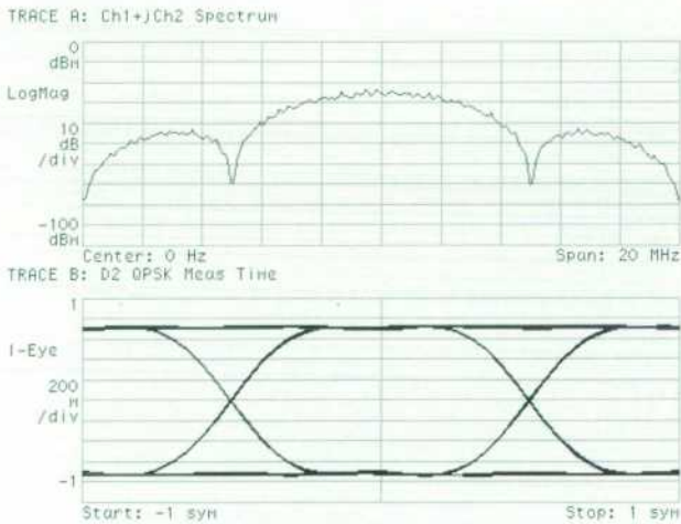
Fig. 1. The upper trace shows the spectrum of a QPSK signal operating at 10 Mbits/s. The lower trace is the eye diagram obtained using the HP 89410A's optional digital demodulator.
