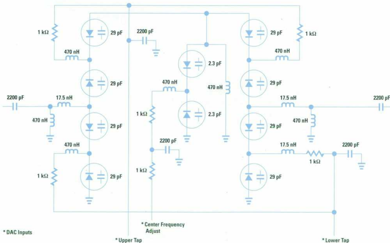
Fig. 13. Circuitry for one pole of the IF bandwidth filter showing the upper and lower tap varactors ganged together.
