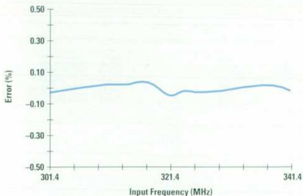
Fig. 27. Discriminator linearity error (percent of full scale).
