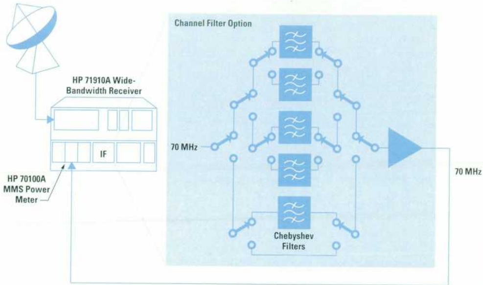
Fig. 7. The HP 71910A channel filters configured with an HP 70100A power meter to measure transponder bandwidth.
