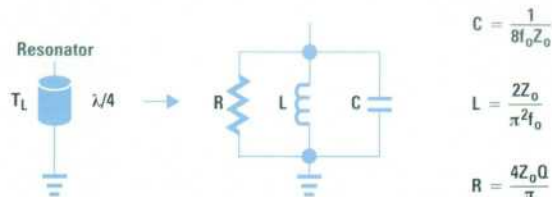
Fig. 6. Equivalent circuit for a ceramic resonator.
