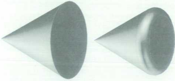
Fig. 3. A torus provides a smooth blending of the edge between a conical surface and a planar surface.
