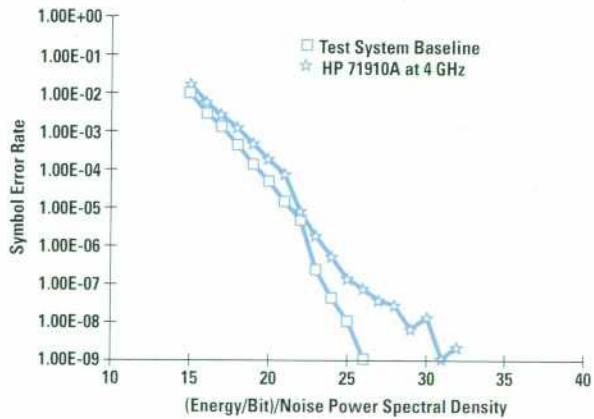
Fig. 8. Results of a 64 QAM 150-Mbit/s bit error rate (BER) test for the HP 71910A.
