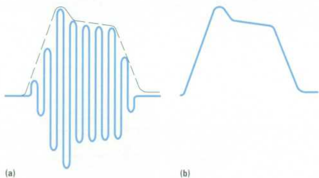
Fig. 17. (a) Input to the linear detector. (b) Output from the linear detector after the carrier is stripped off.
