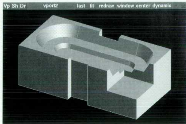
Fig. 12. Part with a tapered, countersunk pocket. The front corner of the block has been cut away to show the tapered pocket.
