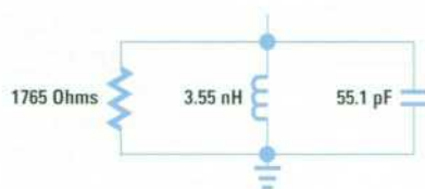
Fig. 7. Circuit values for the ceramic resonator's equivalent circuit.
