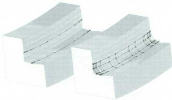
Fig. 13. Creating the geometry of a freeform blend surface: the control polygon of the blend boundaries (left) and the resulting blend surface (right).
