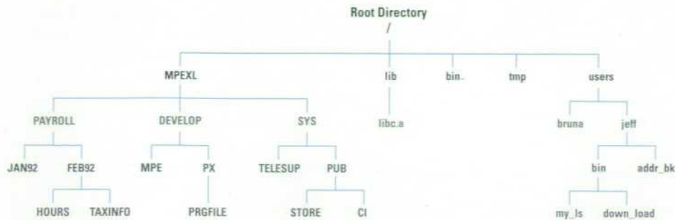
Fig. 5. A directory structure that was rejected for MPE/iX.
