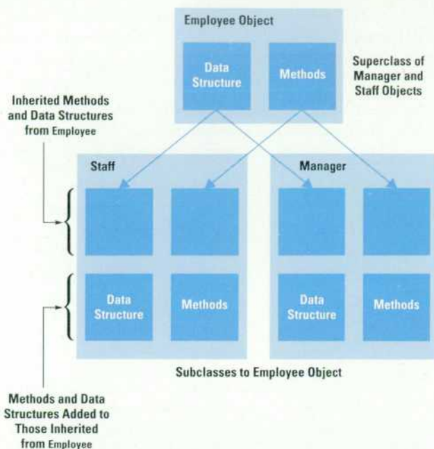
Fig. 5. An illustration of the generalization/specialization data abstraction technique. Here two objects Manager and Staff inherit characteristics from the superclass Employee . They become subclasses when the methods and data structure inherited from Employee is augmented with new methods and data structures in each object.
