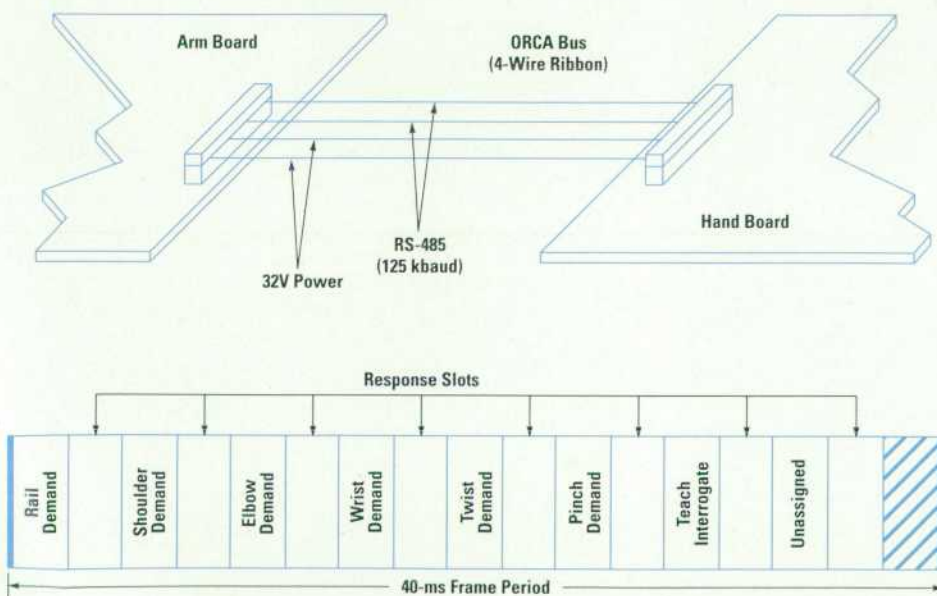
Fig. 6. ORCA bus and data structure.
