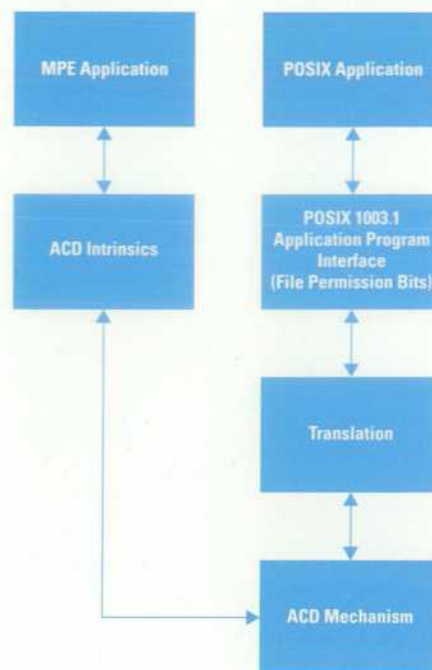
Fig. 8. Access control implementation in MPE/iX. Note that the ACD mechanism is the foundation for both the MPE ACD intrinsics and the POSIX file permission bits.
