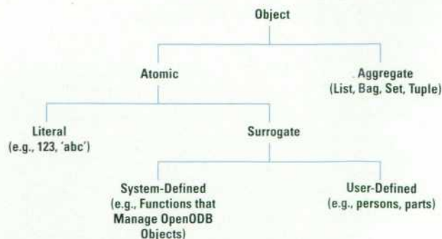
Fig. 6. The taxonomy of OpenODB objects.
