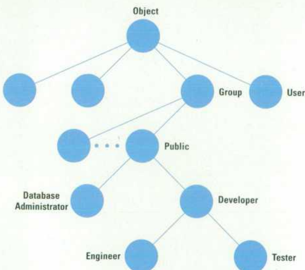
Fig. 8. An example of an access-control hierarchy in OpenODB.
