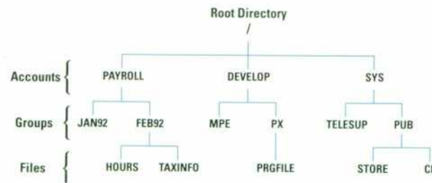
Fig. 2. A typical MPE directory.
