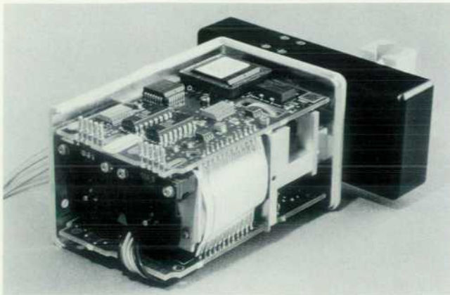
Fig. 4. Interior of robot hand.
