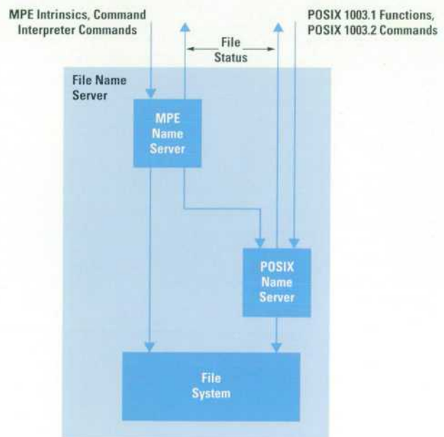
Fig. 7. The POSIX and MPE name servers. The MPE name server escapes to the POSIX name server if the file name begins with . or /.
