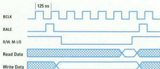
Fig. 3. A typical six-BCLK ISA cycle.
