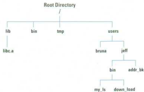
Fig. 3. A typical POSIX directory.
