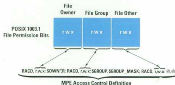
Fig. 9. Mapping between the POSIX 1003.1 file permission bits and the underlying ACD mechanism.
