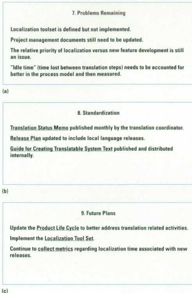
Fig. 5. Panels for the third part of the TQC storyboard for the software translation enhancement project.
