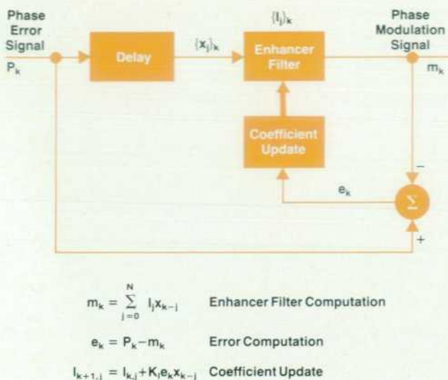
Fig. 15. Adaptive line enhancer enhances coherent signals present in the phase error while suppressing noise.
