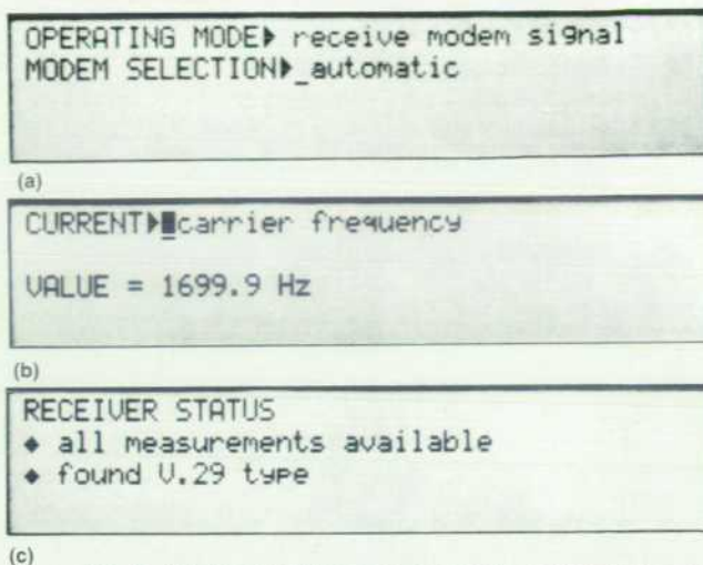
Fig. 6. (a) Active fields allow the user to communicate with the instrument. Each field has a parameter name and a user-selected value. (b) Results pages are used by the instrument to return information to the user. (c) Status fields show various instrument conditions.
