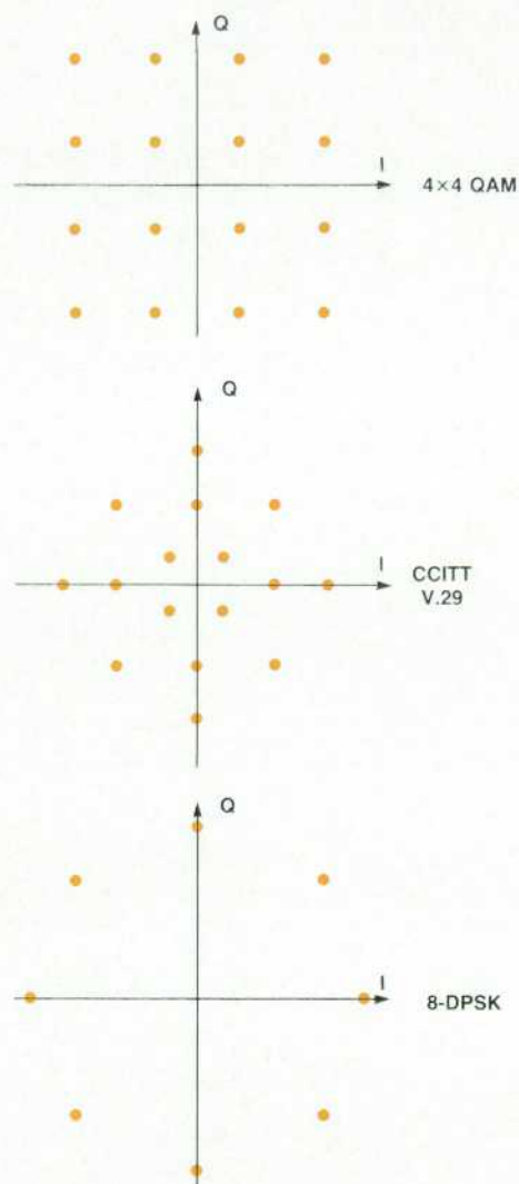
Fig. 3. Typical impairment-free constellation diagrams for various digital modulation schemes. Each point represents one possible combination of in-phase (I) and quadrature (Q) modulation components.
