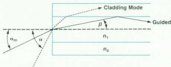
Fig. 2. Only modes with angles smaller than \alpha_m or \beta are guided. Larger angles cause penetration into the cladding, where absorption eventually occurs.
