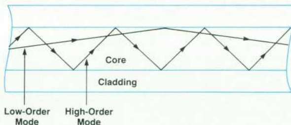
Fig. 1. Mode propagation in a step-index glass fiber. Typically, modes number around 500 for graded-index profiles and around 1000 for step-index profiles.
