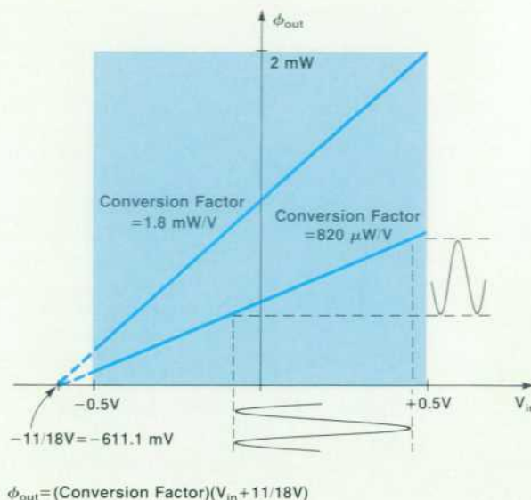
Fig. 4. With external modulation, the user can select the conversion factor in milliwatts, microwatts, or nanowatts of optical output per volt of electrical input.
