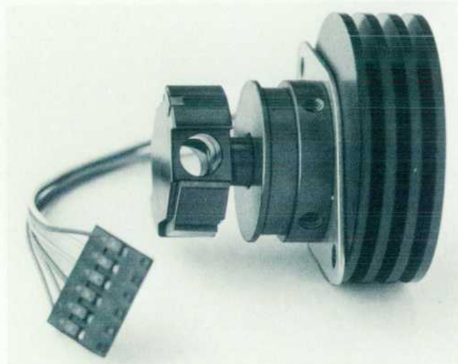
Fig. 18. Step attenuator assembly (0, 20, or 40 dB or \infty ).
