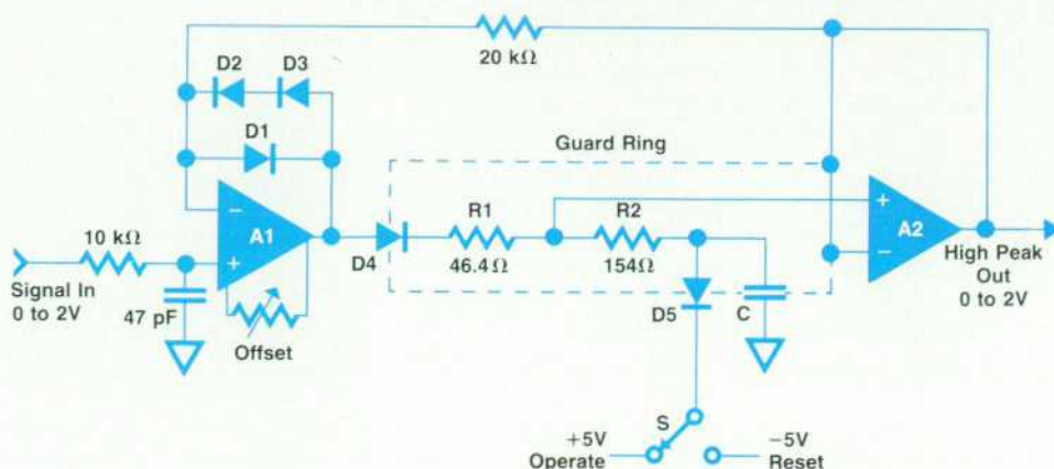
Fig. 10. Schematic diagram of the analog peak reader that detects the high peak level in the low-frequency path of the HP 8151A. For the low peak reader, all diodes are reversed.
