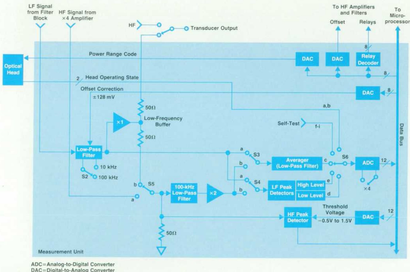
Fig. 9. In the measurement unit of the HP 8151A Optical Pulse Power Meter are the filters, peak detectors, digital-to-analog converters, and analog-to-digital converters that perform all of the analog and digital signal processing in the instrument.
