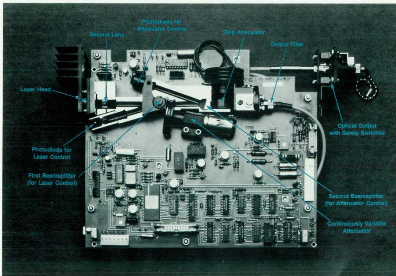
Fig. 13. The laser light is controlled and attenuated within this miniature optical bench. A solid metal block carries the optical elements.
