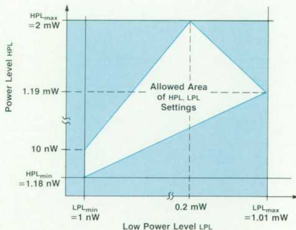
Fig. 12. Range of possible high and low power level settings. Automatic adjustments occur internally to keep the HP 8150A's operation in the allowed range.
