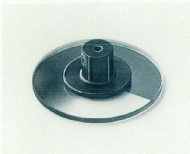
Fig. 17. Continuously variable attenuator disc (0-20 dB).
