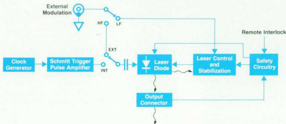
Fig. 1. Block diagram of the optical rise time standard.
