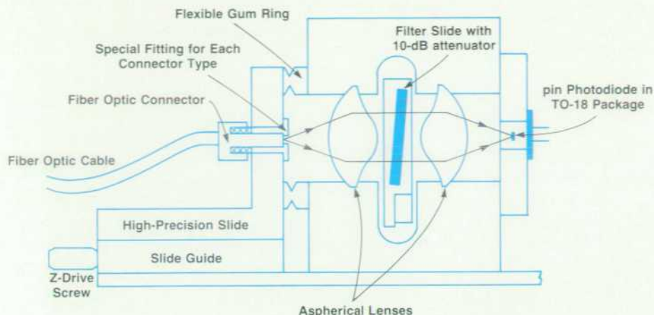
Fig. 5. The HP 81511A Optical Head accommodates different types of fiber optic connectors by using a special fitting for each connector type. The slide carrying the fitting is adjustable with respect to the focal point of the lens system inside the head.
