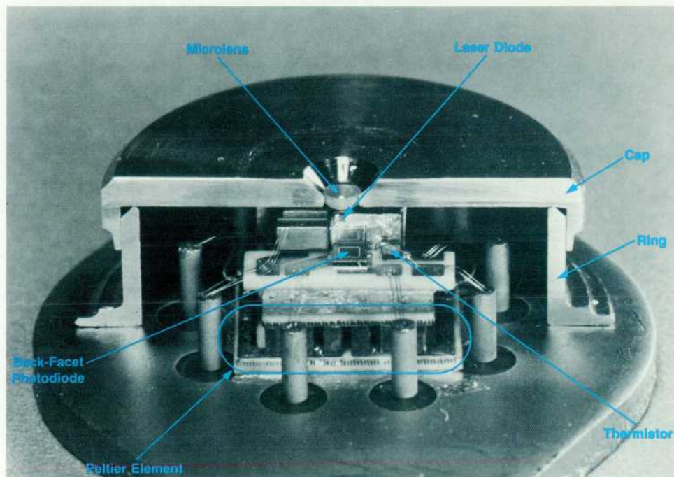
Fig. 8. The laser diode is mounted on a thermoelectric cooler and its temperature is controlled by a regulator circuit. This cutaway view of the laser head shows the Peltier cooler, the photodiode for monitoring the laser's back-facet emission, the thermistor, and the GaAlAs laser diode.
