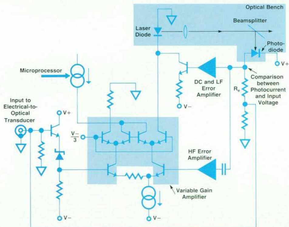
Fig. 9. Simplified schematic of the laser control section that compensates for laser nonlinearity. The front-facet laser radiation (i.e., the actual laser output) is sampled by a beamsplitter and a photodiode. Only highly linear components are used at the error node (comparison point).
