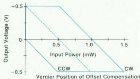
Fig. 2. Offset compensation allows adjustment of the input power that produces a 0\text{V} output.
