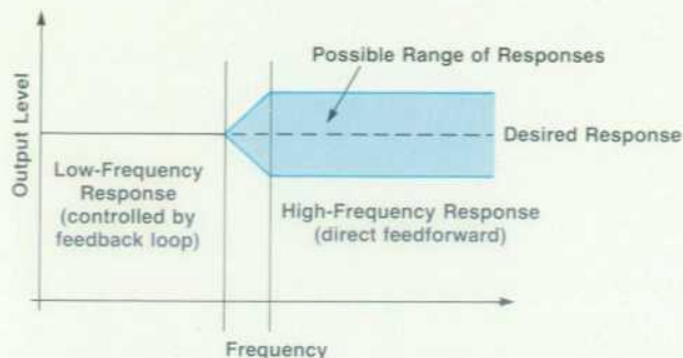
Fig. 10. The laser control section provides closed-loop control of the laser output up to the loop cutoff frequency. Above the loop bandwidth, laser control is open-loop. The closed-loop and open-loop frequency responses must be carefully matched. This is done by a separate laser gain control section.
