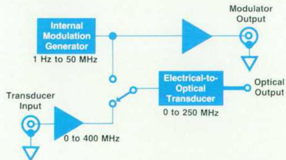
Fig. 3. Simplified block diagram of the HP 8150A Optical Power Source.
