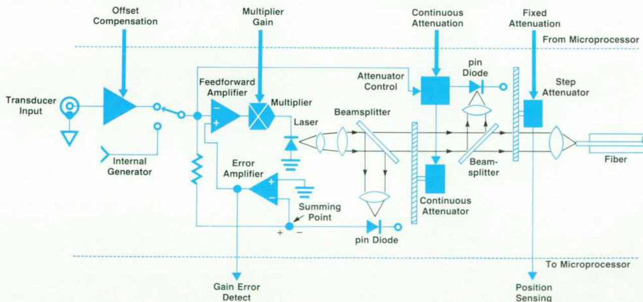
Fig. 5. Block diagram of the electrical-to-optical transducer. Light emitted by the laser diode is controlled by various attenuators and feedback loops.
