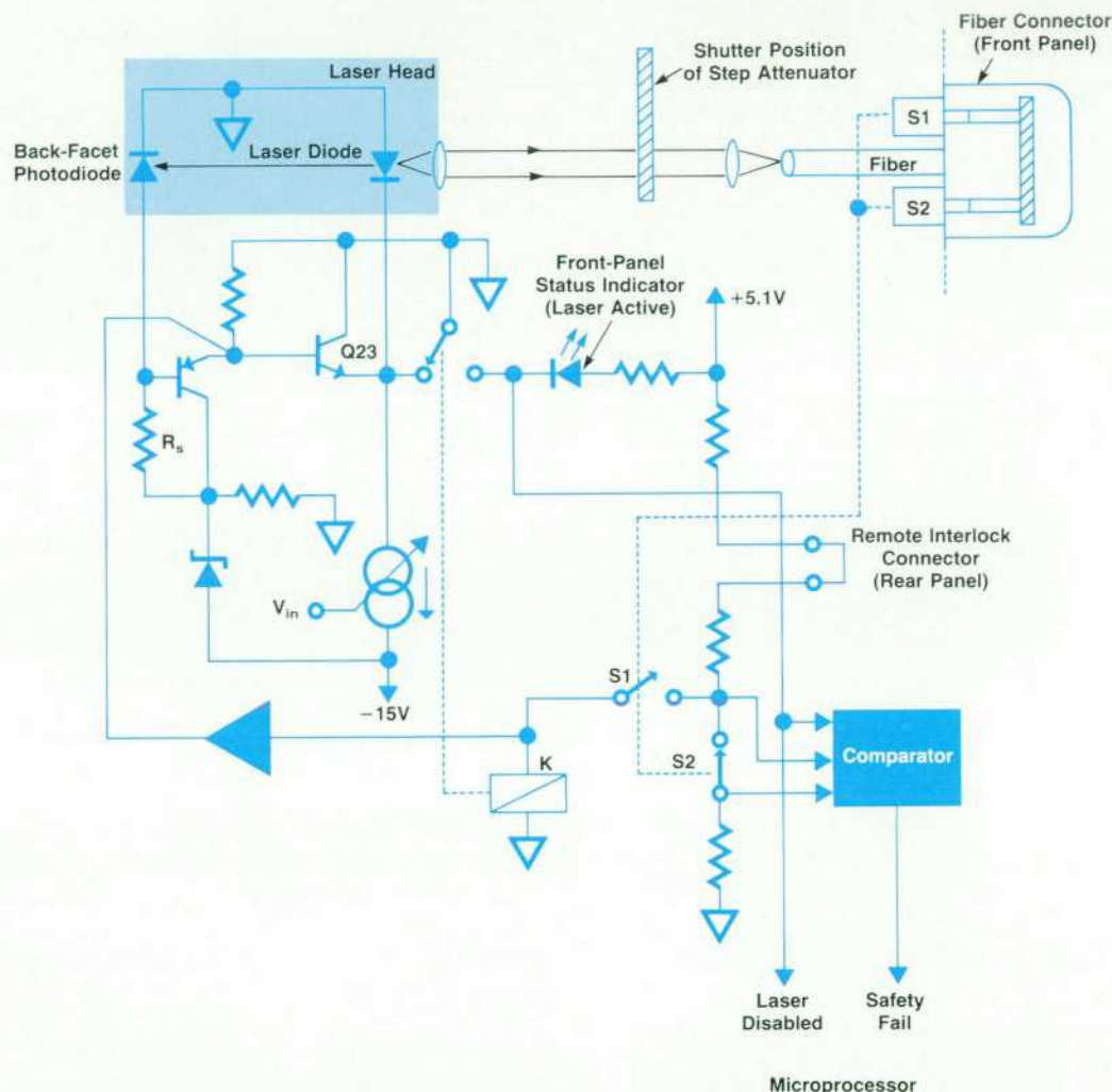
Fig. 15. This laser safety and protection circuit prevents laser damage caused by overdriving the laser. It also shuts off the light output when no optical fiber is connected.
