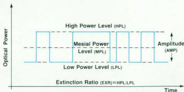
Fig. 2. With internal modulation, the user can modify four parameters of the optical signal. These are the high and low levels, the mesial level, and the extinction ratio.
