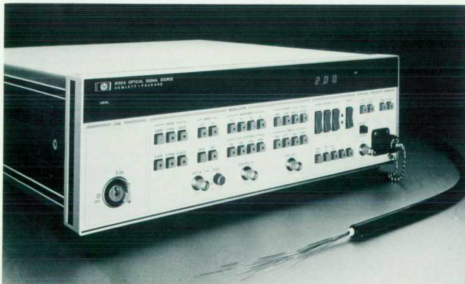
Fig. 1. The HP 8150A Optical Signal Source produces optical power at a wavelength of 850 nm over a range of 1 nW to 2 mW. Power level accuracy is \pm 0.5 dB relative and \pm 1 dB absolute, stability is \pm 0.05 dB, and total harmonic distortion is less than 2%. Internal or external modulation of the optical signal is possible over a frequency range of dc to 250 MHz.
