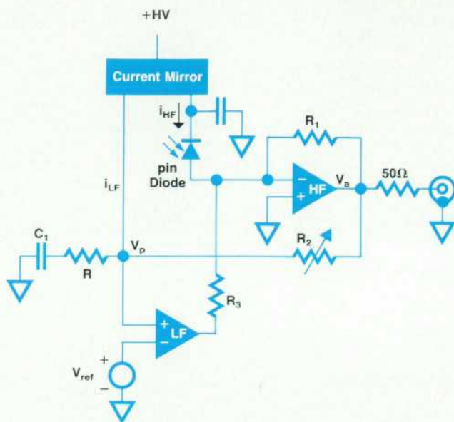
Fig. 3. The optical-to-electrical transducer uses a pin photodiode working into a transimpedance amplifier. The amplifier has two paths, one for high frequencies and one for low.
