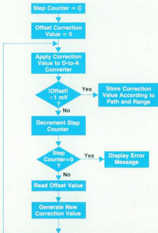
Fig. 13. Flow chart of the offset determination routine.
