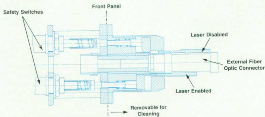
Fig. 19. Cleanable fiber optic output connector with safety switches.
