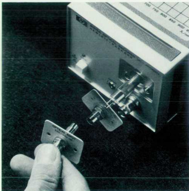
Fig. 5. The optical input connector pulls out for easy cleaning, as shown in this multiple-exposure photograph.
