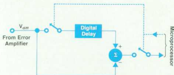
Fig. 11. Matching of closed-loop and open-loop frequency responses is done by modulating the laser with a square wave and monitoring the difference between the actual and the nominal signals. The major element of the control loop is this sample-and-hold-compare circuit. The microprocessor reads its output and adjusts the laser current to find the minimum of the difference signal.
