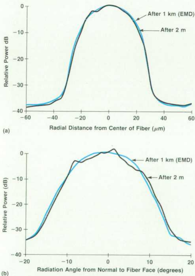
Fig. 14. (a) A near-field scan of the mode distribution 2 meters from the HP 8150A output shows excellent matching with the desired equilibrium mode distribution measured after a 1-km fiber. (b) The far-field scan also shows good matching with the equilibrium mode distribution. The ripple is caused by the speckle pattern on the fiber end, a result of the coherent light of the laser diode.
