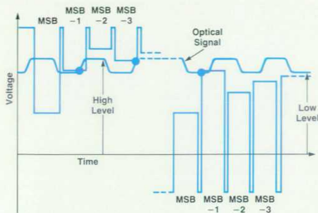
Fig. 12. Using the high-frequency peak detector, the microprocessor executes an algorithm similar to successive approximation to find the highest and lowest peaks of the input signal.
