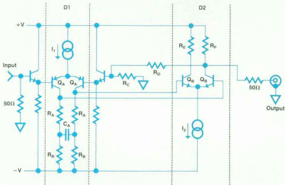
Fig. 7. One of the two identical 6-dB ( \times 4 ) amplifiers in the high-frequency path of the optical pulse power meter.
