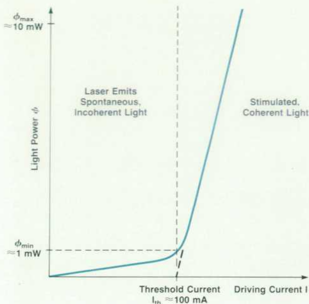
Fig. 6. Typical flux-versus-current curve for a gain-guided laser diode. Note the minimum, or pedestal, light power \phi_{\min} .
