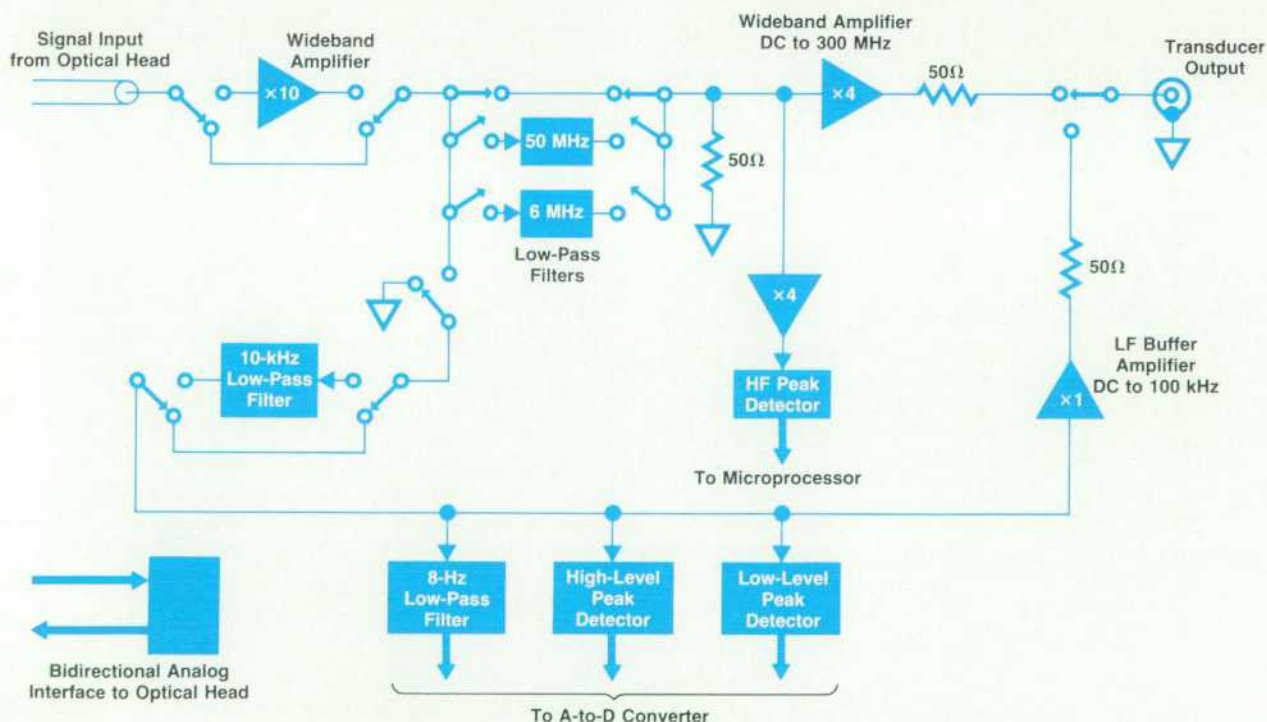
Fig. 6. Like the optical head, the HP 8151A Optical Pulse Power Meter has two paths, a wideband path and a high-sensitivity path. Peak detectors measure the high and low signal levels, and an 8-Hz low-pass filter produces an average signal.
