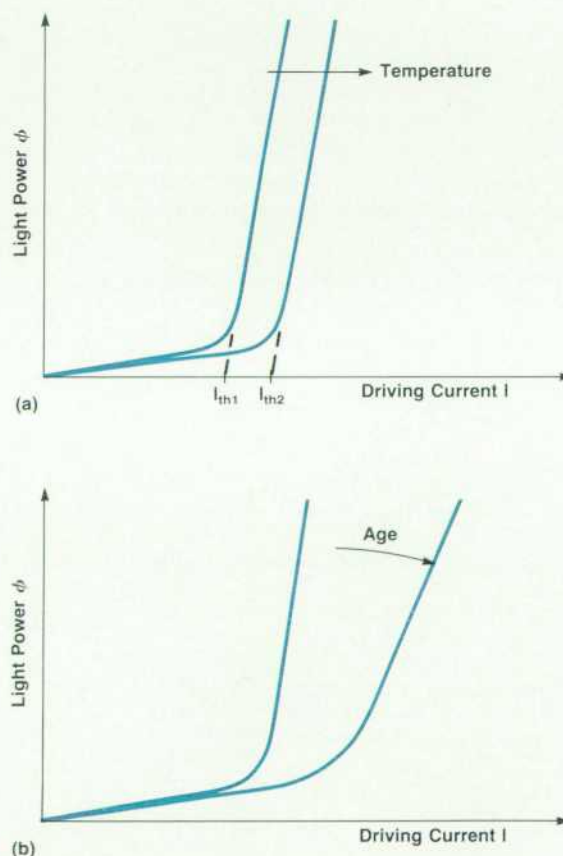
Fig. 7. (a) Temperature dependence of laser diodes. The typical temperature coefficient of the threshold current is 1^\circ\text{C} . (b) Aging behavior of laser diodes. With time, the threshold current increases and the differential efficiency decreases.
