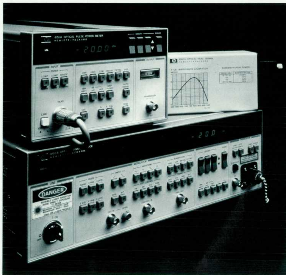
Fig. 1. Two new products, the HP 8150A Optical Signal Source (bottom) and the HP 8151A Optical Pulse Power Meter (top left, shown with the HP 81511A Optical Head), are precise, fully programmable stimulus and response-measuring instruments for design and production testing of fiber optic devices and systems at short wavelengths.
