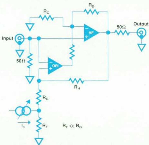
Fig. 8. To control the low-frequency gain of the 6-dB wide-band amplifiers, operational amplifier OPI is added. Low-frequency gain is determined by the ratio R_H/R_G . Current source I_3 is adjusted to compensate for system offsets.
