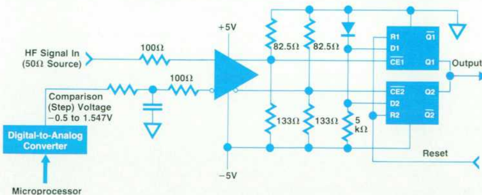
Fig. 11. High-frequency peak detector circuit. This circuit can detect pulses as narrow as 4 ns at a repetition rate as low as 200 Hz.
