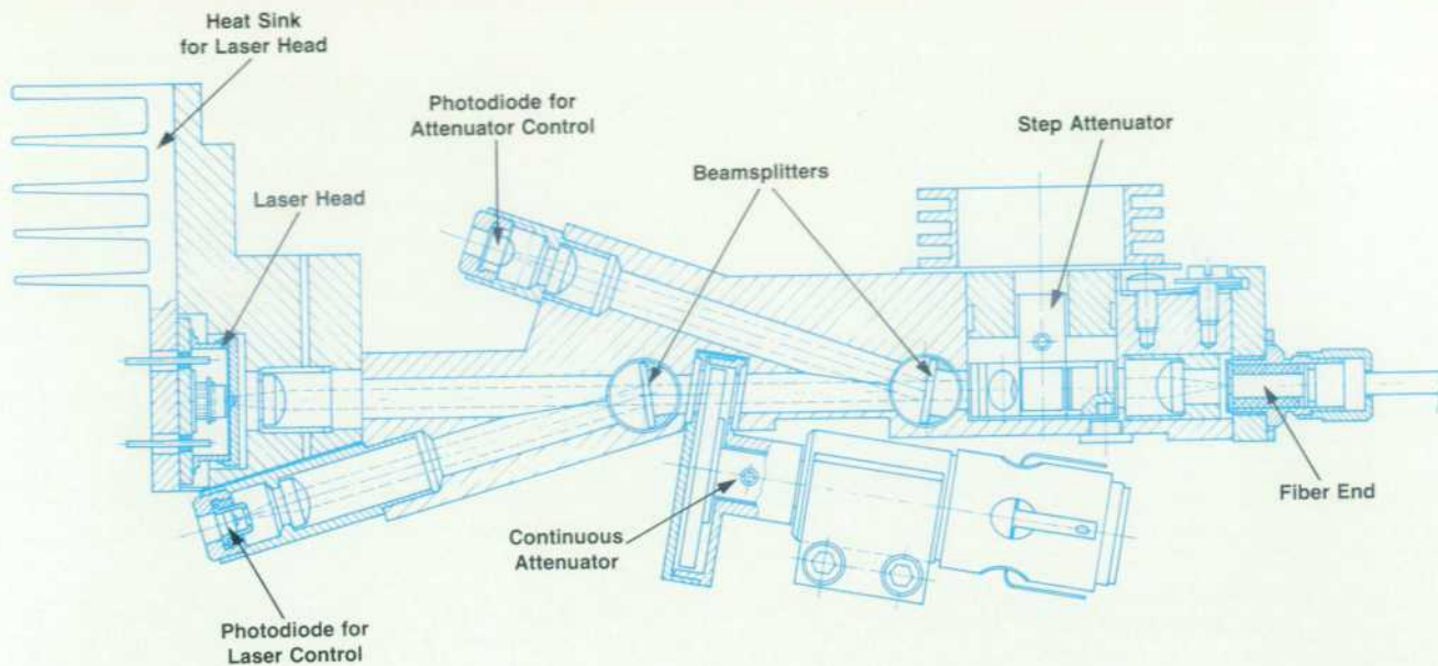
Fig. 16. Cross section of the optical bench.
