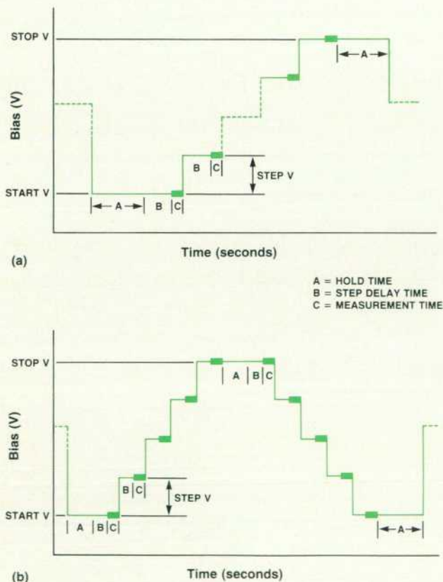
Fig. 20. Single staircase (a) and double staircase (b) dc bias sweep parameters.
