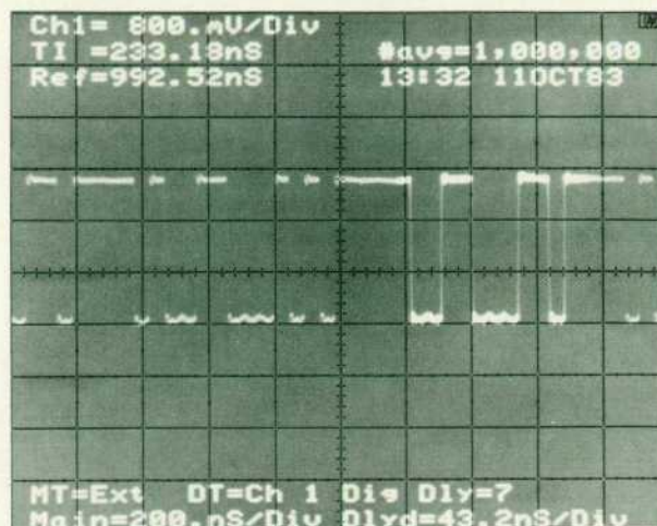
Fig. 2. Measurement of the pulse width of the seventh pulse of a train of pulses.
