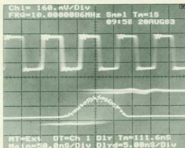
Fig. 4. The phase modulated 10-MHz reference signal (top), an expanded view of one of its leading edges (middle), and a histogram showing the Gaussian distribution of the relative phase shift at the 50% point on the leading edge.
