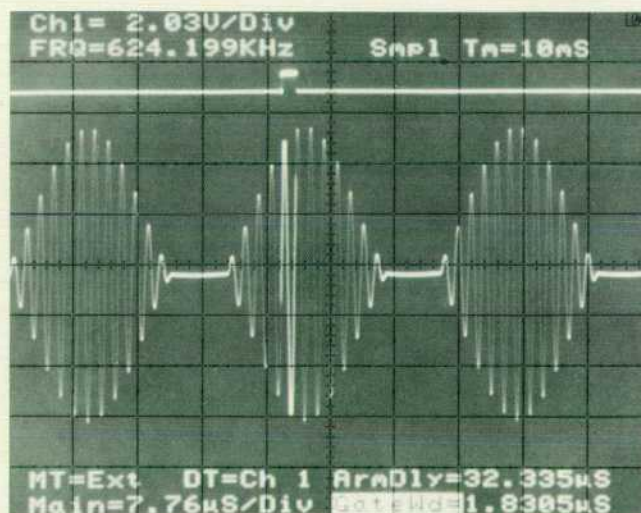
Fig. 5. A gated frequency measurement on a burst is performed using the intensified portion (i.e., the delayed sweep gate) to window the measurement.
