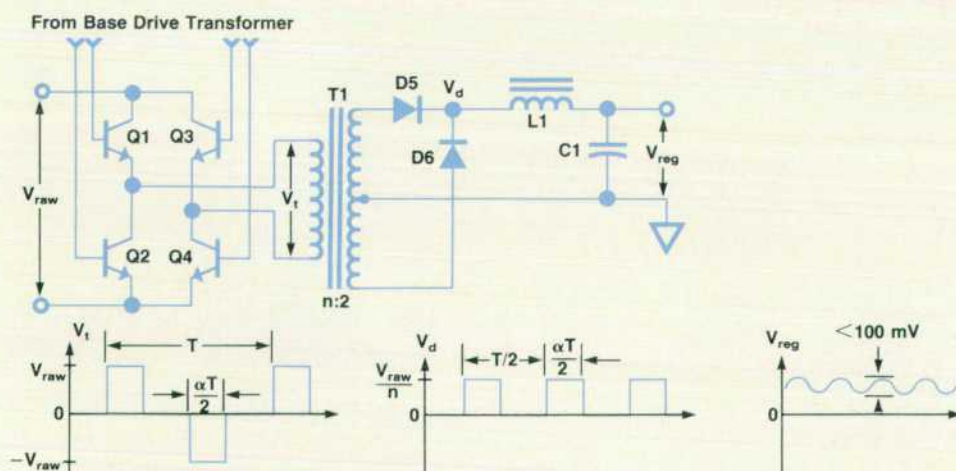
Fig. 2. Basic circuit diagram of the primary switching regulator circuit. See Fig. 3 for more details.
