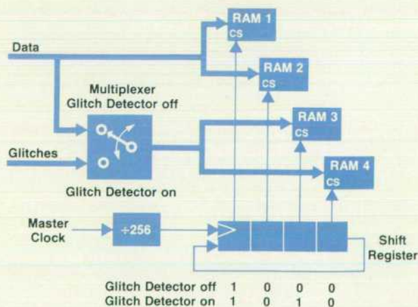
Fig. 9. For glitch detection, the high-speed RAM is split into data and glitch memories of equal size.
