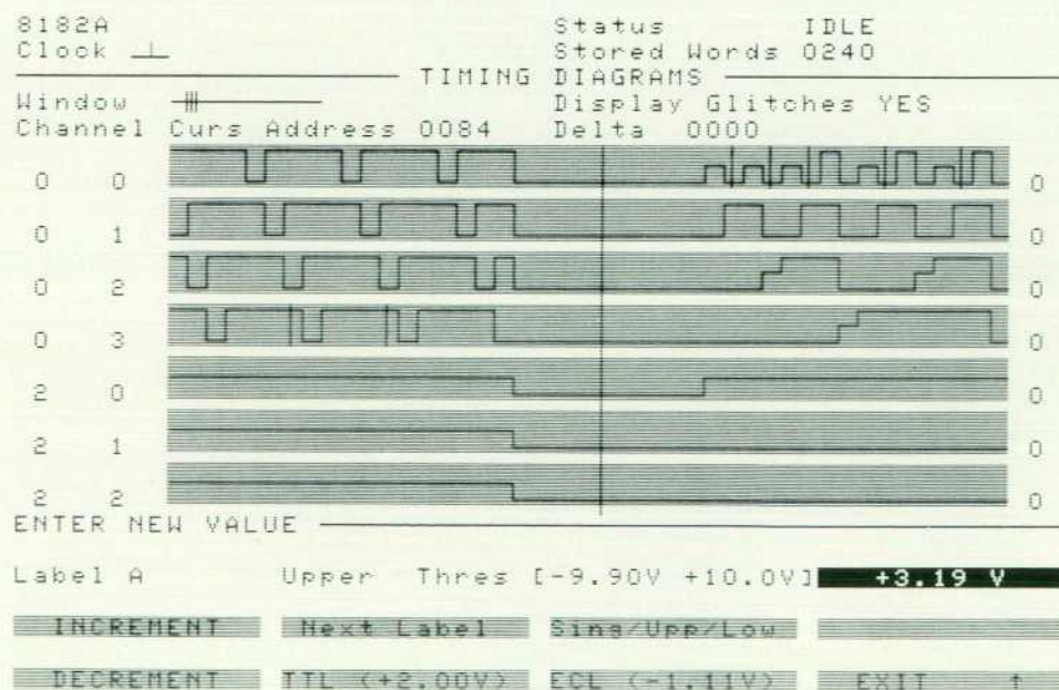
Fig. 3. When changing measurement parameters during a measurement, the display can be split into two areas, one of which shows control page parameters in the softkey area. Here the timing page is displayed while the probe threshold is being changed.
