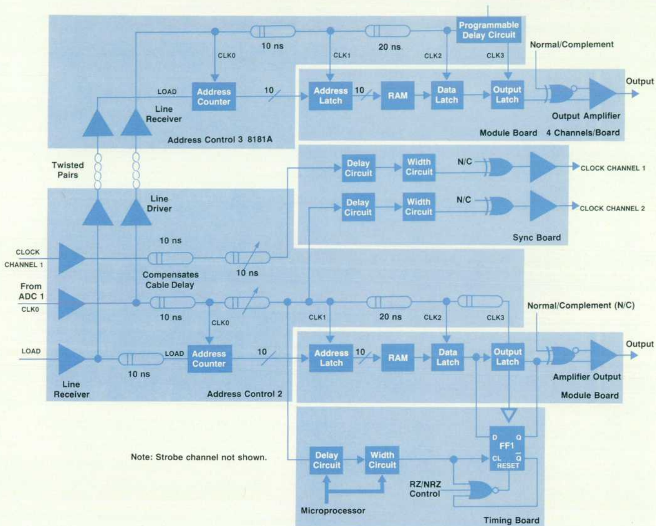
Fig. 4. 8180A/8181A timing and signal distribution.
