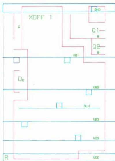
Fig. 2. The ASAP design starts with the simple symbols on the far left and progresses to a more detailed symbolic representation which is translated into the geometrical layout used to fabricate the circuit shown on the far right.
