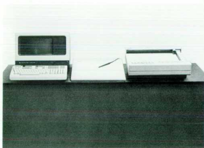
Fig. 1. DRAW circuit design station consists of an interactive graphics terminal, a digitizing tablet, and a four-color plotter, all tied to a timeshared computer. DRAW is a graphics editor designed for editing schematics.
