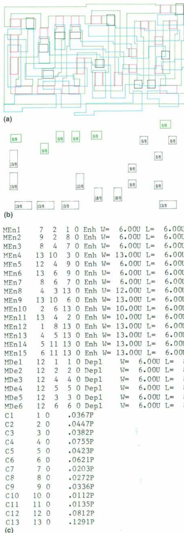
Fig. 2. Extraction of a NMOS full-bit adder. (a) Input artwork. (b) Transistors shown with width and length dimensions. (c) Circuit schematic generated for input to SPICE simulator.
