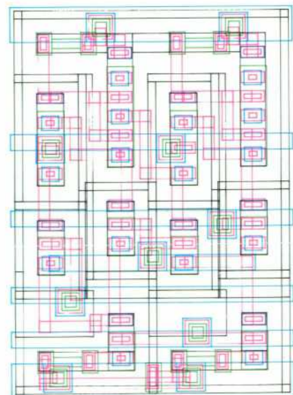
Fig. 2. The ASAP design starts with the simple symbols on the far left and progresses to a more detailed symbolic representation which is translated into the geometrical layout used to fabricate the circuit shown on the far right.
