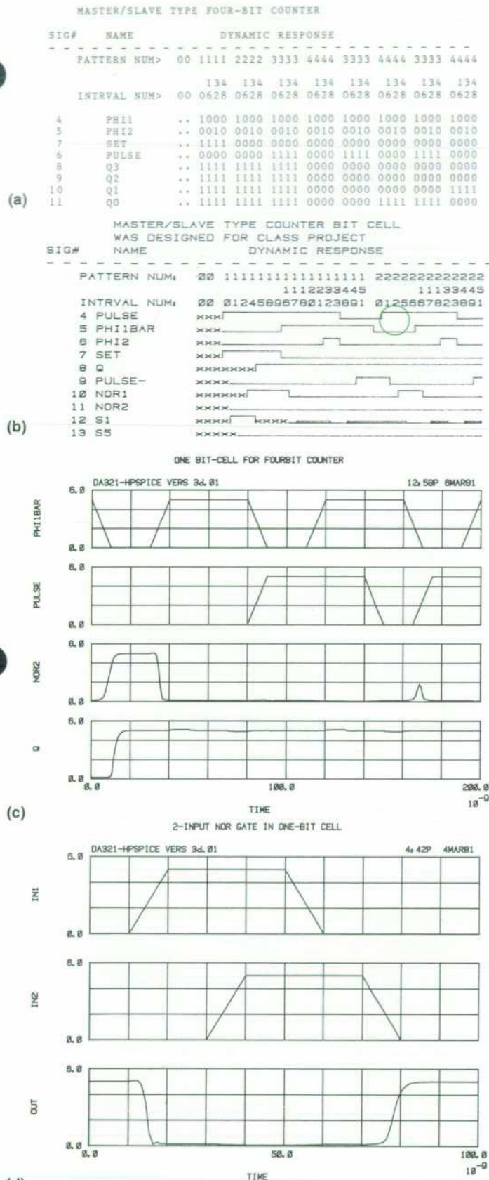
Fig. 4. TESTAID-IC and HP-SPICE plots. (a) Functional behavior of a four-bit counter. (b) Logic response of a one-bit counter cell. (c) HP-SPICE plot of a one-bit cell response, showing a toggle failure. (d) HP-SPICE plot of a two-input NOR gate response.
