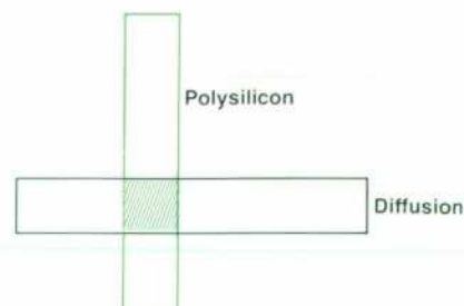
Fig. 1. Isolation of an NMOS transistor gate.
