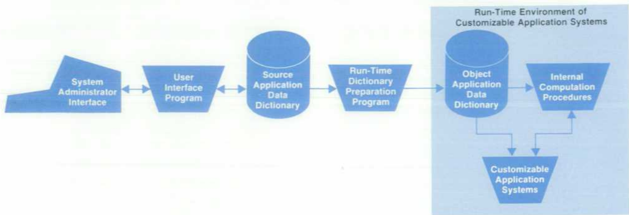
Fig. 3. The Application Customizer consists of three major components: 1) the user interface program, 2) a set of routines that perform data conversions, computations, and comparisons on customizable data fields and structures, and 3) a run-time application data dictionary preparation program.
