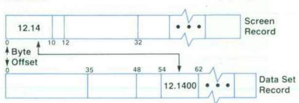
Fig. 8. An example of the operation of the MOVE CORRESPONDING Customizer intrinsic. See text for details.
