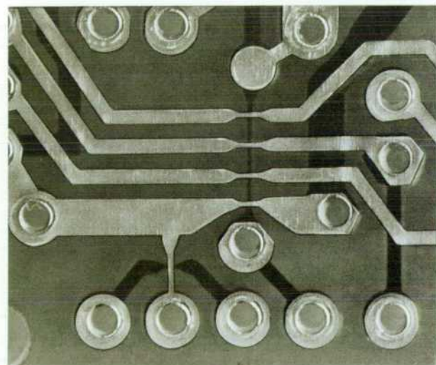
Fig. 5. Stray capacitance between overlapping traces on the thin flexible substrate is reduced by necking down the overlapping traces. When needed, capacitors are easily formed (circular area without hole).
