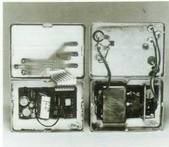
Fig. 4. The sculptured flexible circuit interconnect of the 10811B (left) is a significant improvement over the older 10544C (right).
