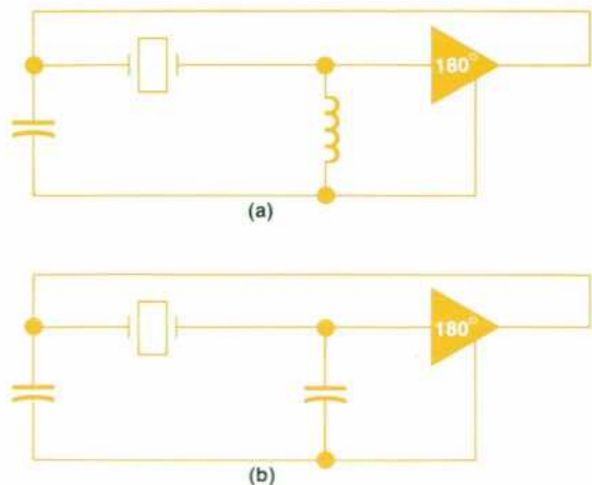
Fig. 8. Equivalent circuits for the mode-suppression circuit of Fig. 7. Top: low and high-frequency equivalent circuit. Bottom: passband equivalent circuit.
