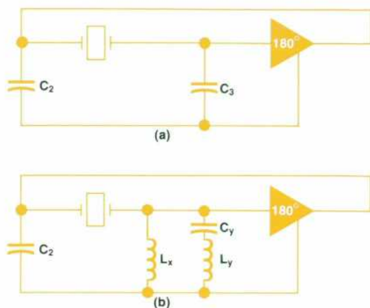
Fig. 7. The SC-cut crystal in the 10811A/B Oscillator is mode-suppressed to allow only C-mode operation. This diagram shows a standard Colpitts-type oscillator (top) and the same oscillator with mode suppression.
