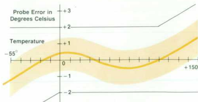
Fig. 4. Typical 10023A error curve with possible unit-to-unit variations (shaded band).
