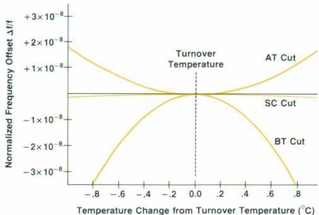
Fig. 1. Comparing the SC-cut crystal's temperature performance with that of two other common cuts, AT and BT.
