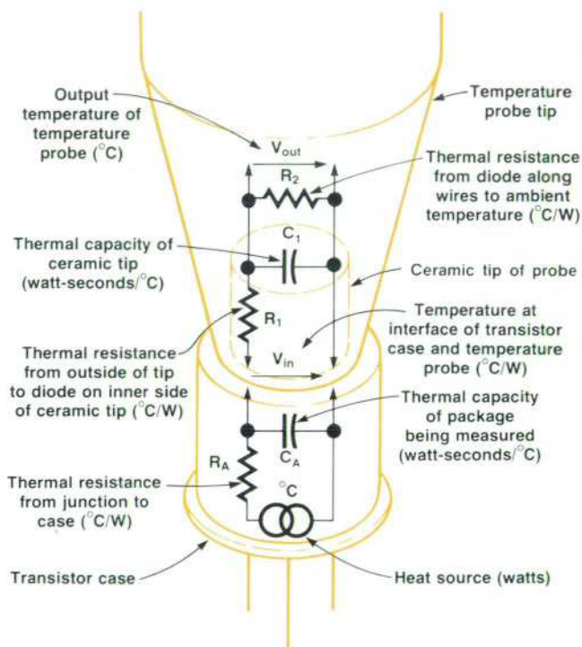
Fig. 2. Simplified electrical analog of the problem of measuring the temperature of a transistor with a probe.
