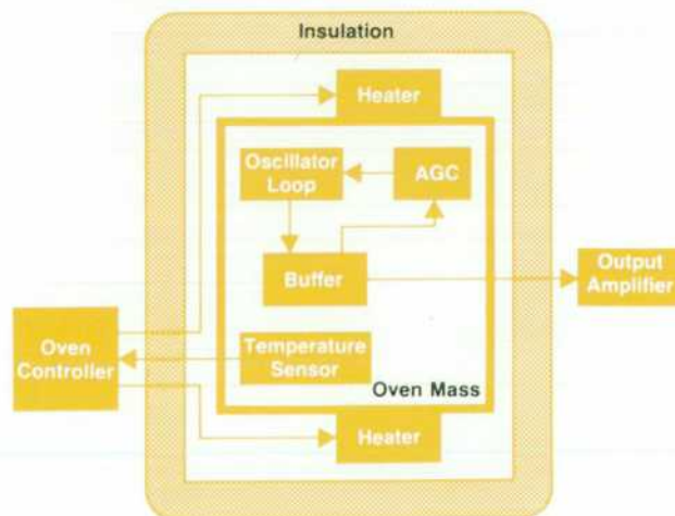
Fig. 6. Block diagram of the 10811A/B Oscillator. The oscillator loop includes a 10-MHz SC-cut quartz crystal.
