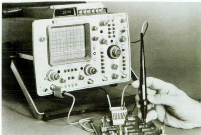
Fig. 1. Model 10023A Temperature Probe gives fast indications of surface temperatures on many general-purpose digital multimeters and HP 1700 Series Option 034/035 Oscilloscopes.
