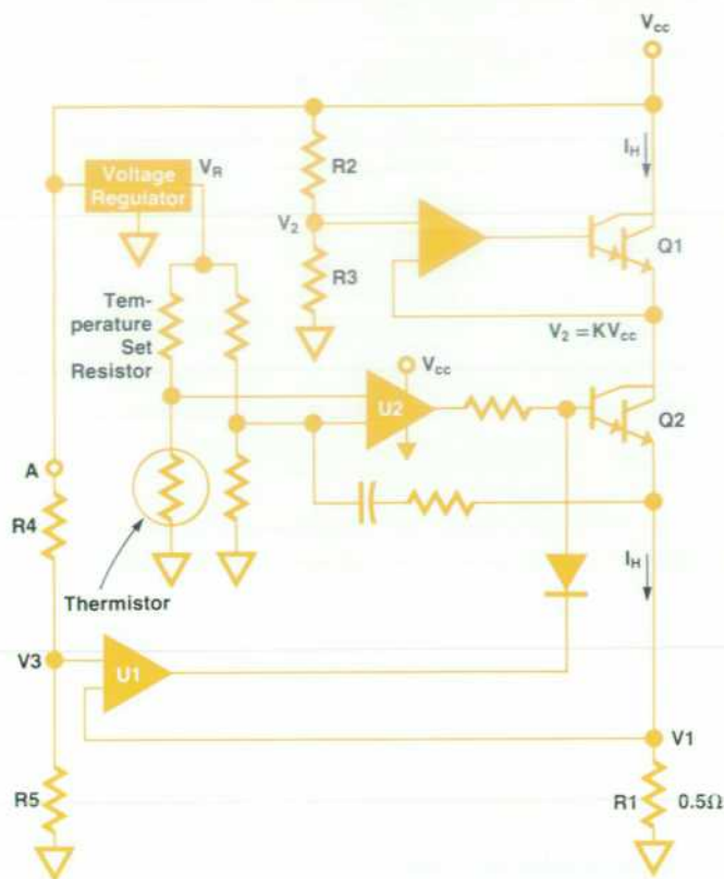
Fig. 10. 10811A/B oven controller block diagram. Two heater transistors heat the oven using direct current only. Overall power consumption is less than two watts in still air at 25°C.
