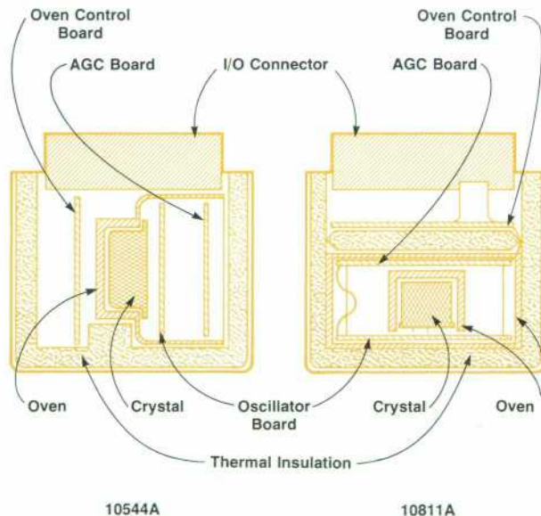
Fig. 1. Cross-sections of the new 10811A Oscillator and the older 10544A.
