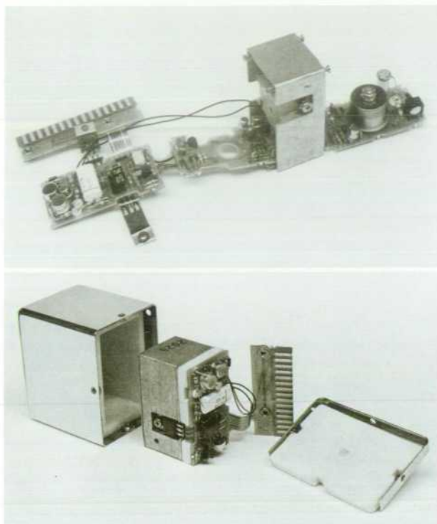
Fig. 3. Final assembly of 10811A/B Oscillator.
