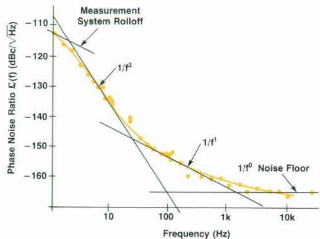
Fig. 2. Typical 10811A/B phase noise plot, showing the noise processes responsible for the overall phase noise.
