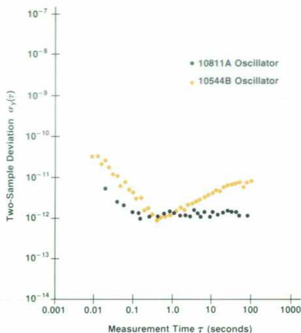
Fig. 3. Time domain stability (short-term) measurements of two 10811A Oscillators and two 10544B's (an older design).
