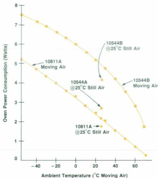
Fig. 4. Steady-state oven power of the 10811A compared with that of the 10544A/B.
