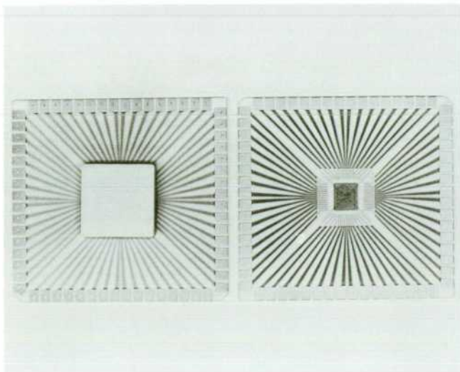
Fig. 4. The VCC is packaged on a 64-pin leadless ceramic substrate measuring 44 mm by 47 mm.
