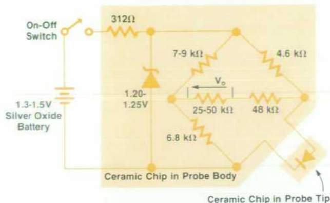
Fig. 3. Simplified schematic of the 10023A Temperature Probe.
