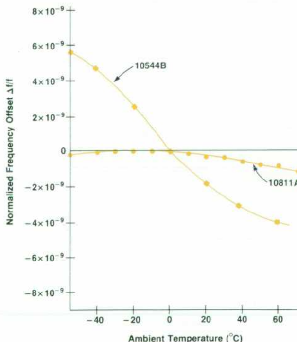
Fig. 5. The new 10811A/B Oscillator's frequency is much less sensitive to ambient temperature than the older 10544B's.
