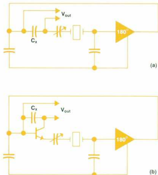
Fig. 9. Phase noise is sensitive to the method of extracting the signal from the oscillator. (a) Method used in the 10544A/B/C. (b) Improved 10811A/B method.
