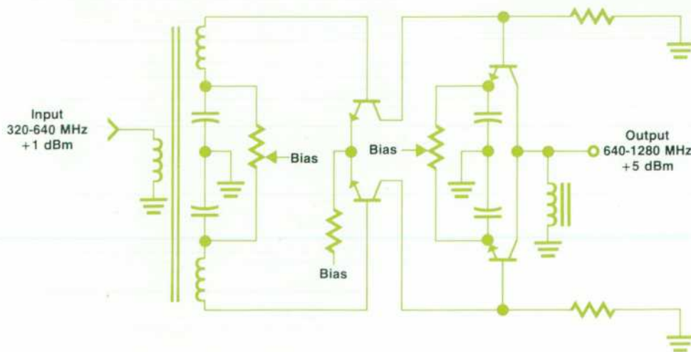
Fig. 6. Active doubler provides better balance and lower subharmonics than a diode rectifier. It also provides gain instead of loss.
