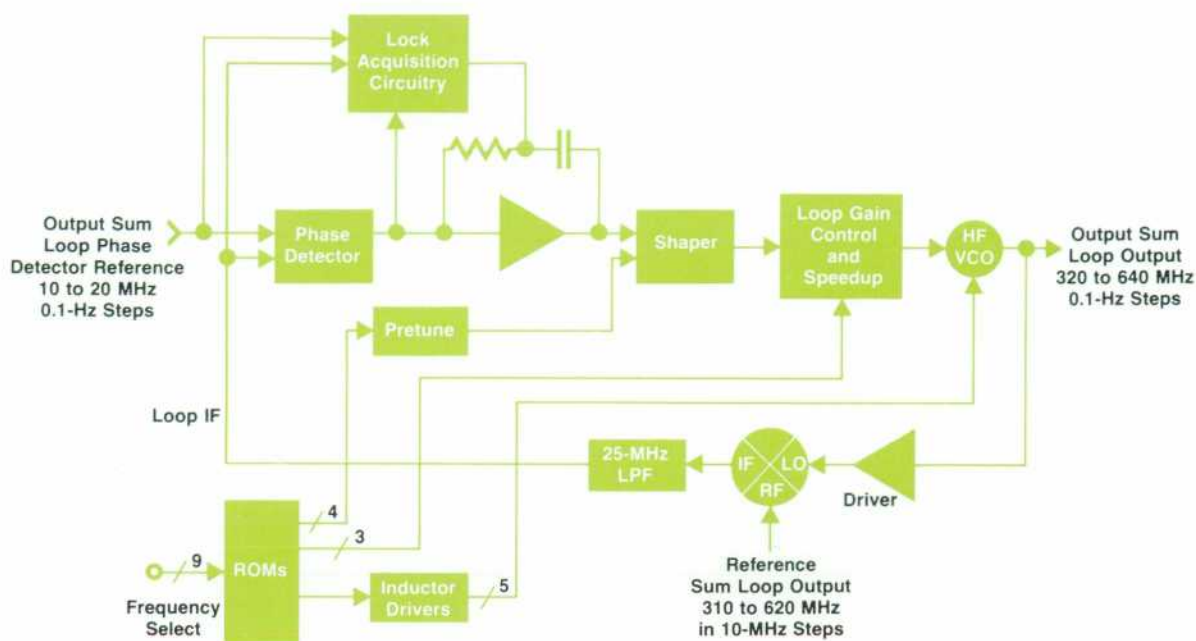
Fig. 4. Simplified block diagram of the output sum loop, high-frequency voltage-controlled oscillator (HF VCO), and ROM controller.
