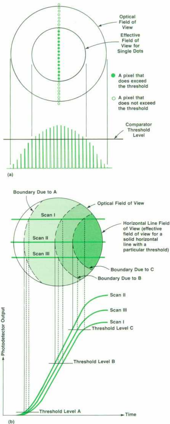
Fig. 3. (a) Single-dot field of view. Because each pixel in a vertical line is separated in time by the period between adjacent scan lines, distinct signal peaks are detected for each pixel in the effective field of view. (b) Horizontal-line field of view. Here the light emitted by each pixel in a horizontal line is added to the light from other pixels in the field of view determined by the threshold level. As the threshold is increased from Level A to Level B and to Level C, the effective field of view diminishes as shown. The center of the horizontal-line field of view is offset to the right because of the light summation required to exceed the higher threshold level.
