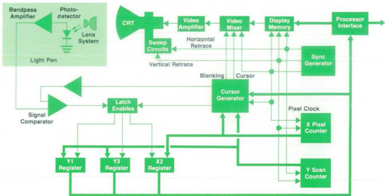
Fig. 2. Block diagram of light pen system in the 9845C Computer.
