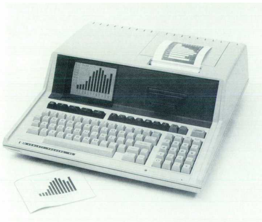
Fig. 1. The HP-85 Personal Computer uses BASIC language programming and operating commands that are permanently resident in the system firmware. Contained in a single package are all of the elements for a small computer system—keyboard entry, tape mass storage, CRT display, and a thermal printer. The inverse video display mode is shown with the associated printer copy at the upper right. In the left foreground is the printer copy for the normal white-on-black display mode.
