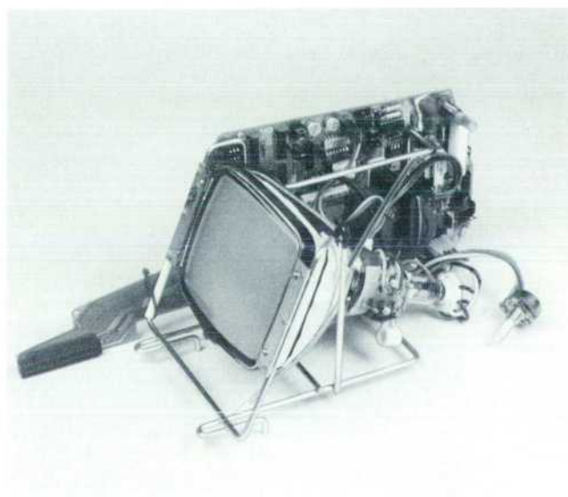
Fig. 1. Photo of CRT subassembly. This unit contains a 127-mm CRT with associated control electronics and can be independently tested before final assembly into an HP-85 system.
