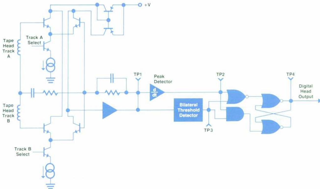
Fig. 6. Schematic for the tape read/write amplifier and detector. Some components are shared for both tape tracks. Tracks are selected by gating the current source for the differential pair associated with the track selected.
