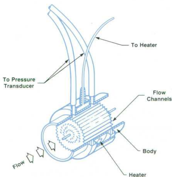
Fig. 4. Resistance to air flow in the pneumotach generates a pressure differential that is proportional to flow rate.
