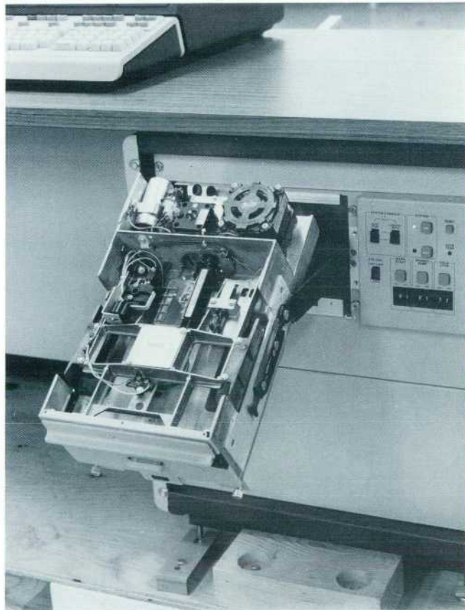
Fig. 3. Flexible disc is mounted on slides that extend and rotate to provide easy access to the top and bottom for service.
