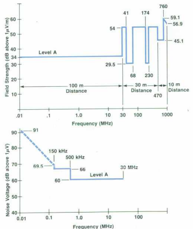
Fig. 1. Radiated and conducted emission limits specified by VDE 0871/6.78.
