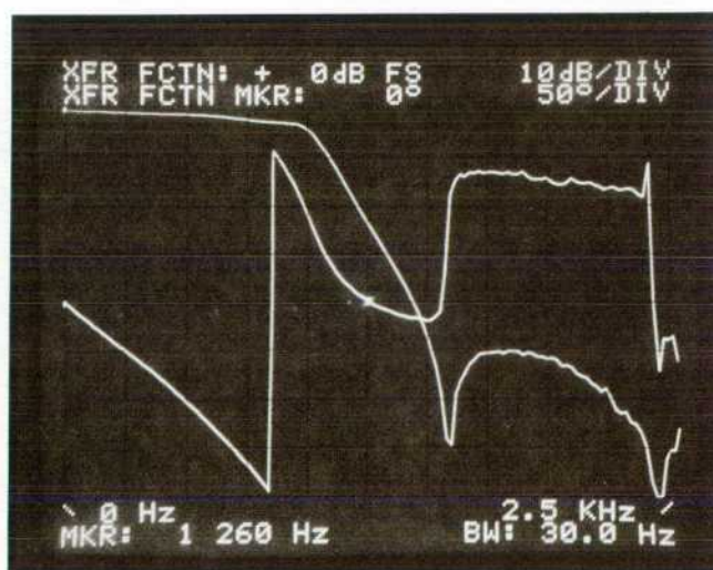
Fig. 3. Model 3582A obtains transfer functions, both magnitude and phase, by relating the signal at the output of a device to the signal at the input. The transfer function can be measured over frequency spans as narrow as 5 Hz anywhere within the 25-kHz range of the analyzer.
