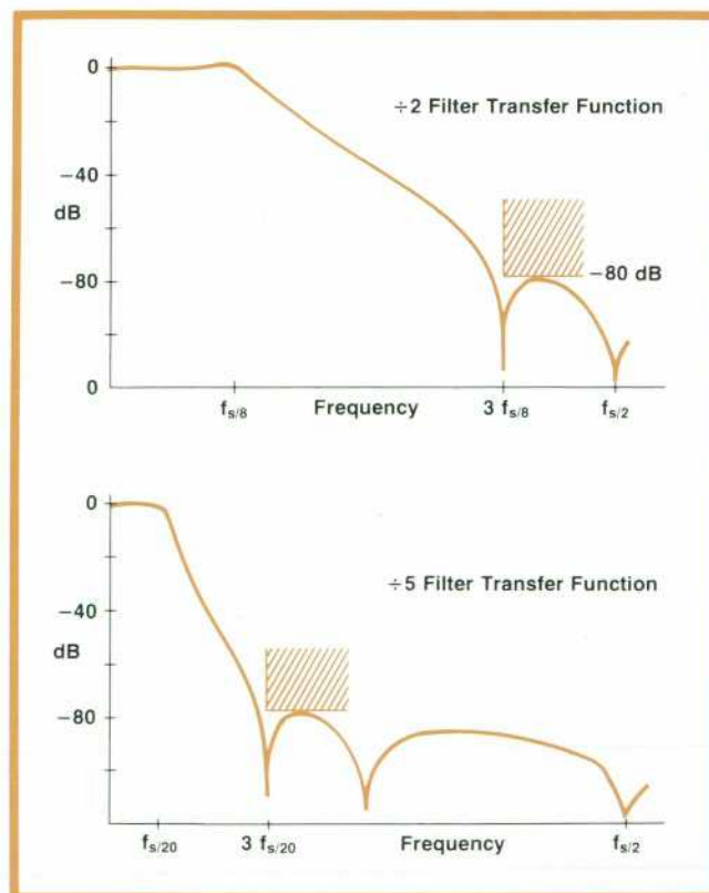
Fig. 6. Transfer functions of the decimation filter selected with the help of a computer iterative procedure. The procedure derived the functions using pole-zero positions selected from those plotted in Fig. 5b.
