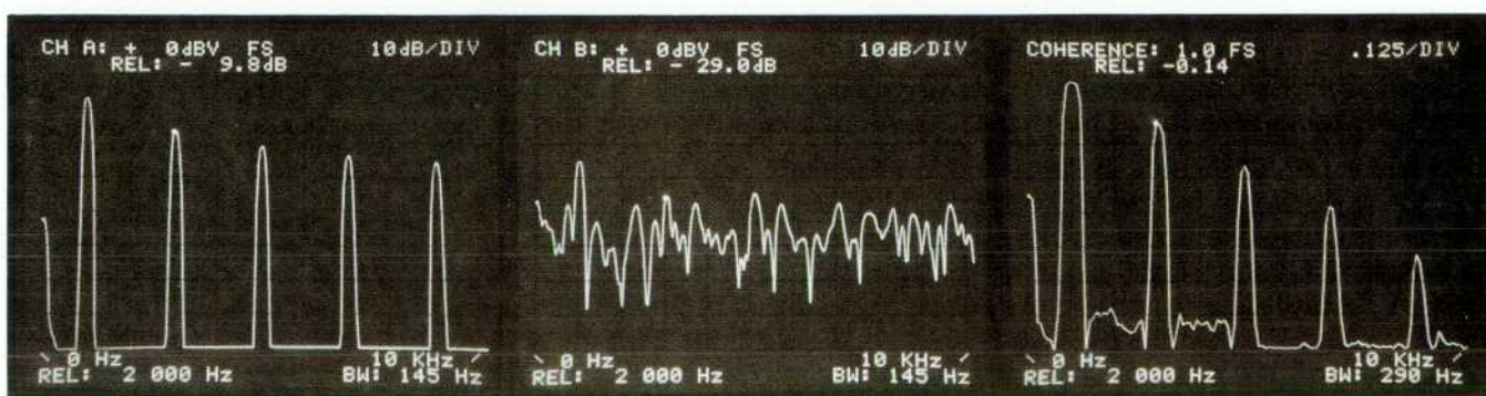
Fig. 5. The coherence function (right) gives a measure of the fraction of power at each frequency in the signal at the output of a device (center) that is caused by the signal at the input (left). Among other uses, this can indicate the validity of a transfer function measurement by showing how much output power comes from sources other than the driving signal.
