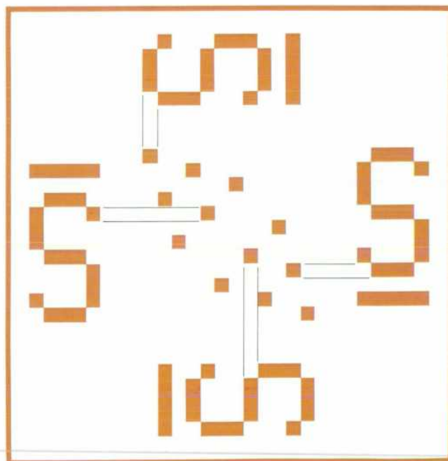
Fig. 5. Dot matrix printhead resistors are arranged in a diamond pattern to allow printing in any of the four orthogonal directions, with or without underline.
