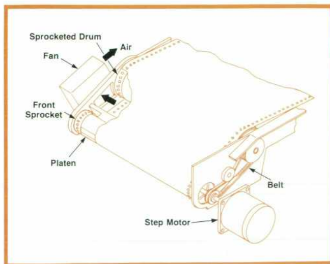
Fig. 10 Sprocketed drive system provides accuracy, repeatability, and reliability. The drive is bidirectional; paper can back up as much as five metres. Repeatability is 0.25 mm from any point in any direction.
