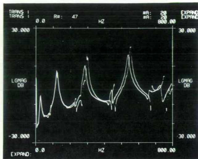
Fig. 11. Measurements before and after adding mass to the steel plate. Extra mass decreases the amplitudes and frequencies of the resonances.
