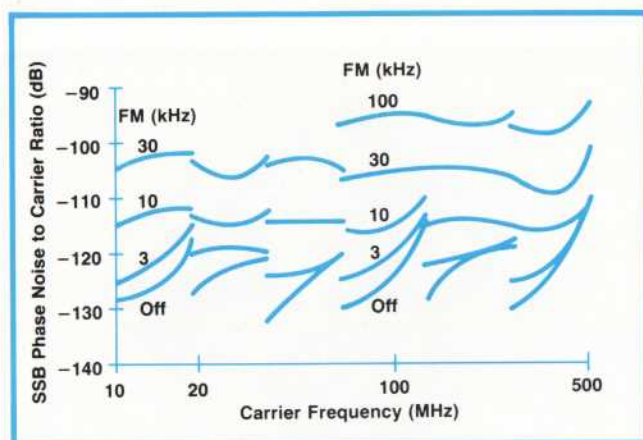
Fig. 6. Typical 8654B phase noise performance, shown as SSB signal-to-noise ratio in a 1-Hz bandwidth 20 kHz away from the carrier. Carrier power is +3 dBm. With FM off, phase noise is similar to that of the 8654A (see ref. 1). With the FM switch in the EXT position, phase noise degrades because of FM modulator noise. At an output power of -7 dBm, noise degrades typically less than 6 dB.
