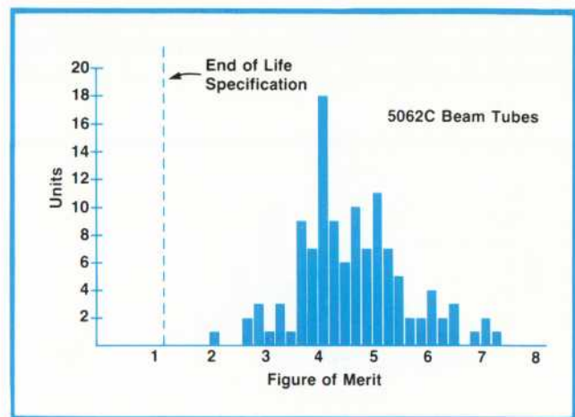
Fig. 9. Figure of merit performance of 5062C's compared to specified end-of-life performance. Figure of merit remains nearly constant until end of life is near.
