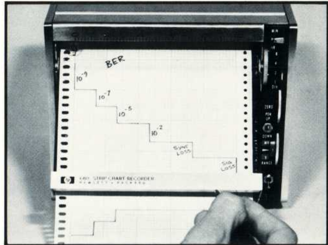
Fig. 9. Pen deflection of the optional strip-chart recorder is proportional to N , the exponent of the bit-error rate where bit-error rate is expressed in the form A.B \times 10^{-N} . It also responds to sync loss and signal loss.
