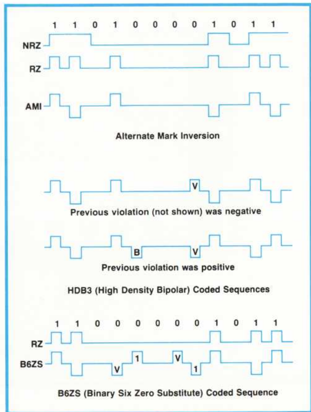
Fig. 4. Output formats of Model 3780A conform to standard practice. The AMI (alternate mark inversion) coding is a three-level code that alternates the polarity of RZ pulses to eliminate any dc component in the average voltage level. HDB3 (high density bipolar) code eliminates long strings of 0's for the benefit of clock recovery circuits by substituting 000V or B00V for four consecutive 0's, where V is an intentional code violation and B is a mark that is inserted to force these violations to alternate in sign. B6ZS (binary six zero substitute) code is similar but substitutes 0V10V1 for runs of six 0's.
