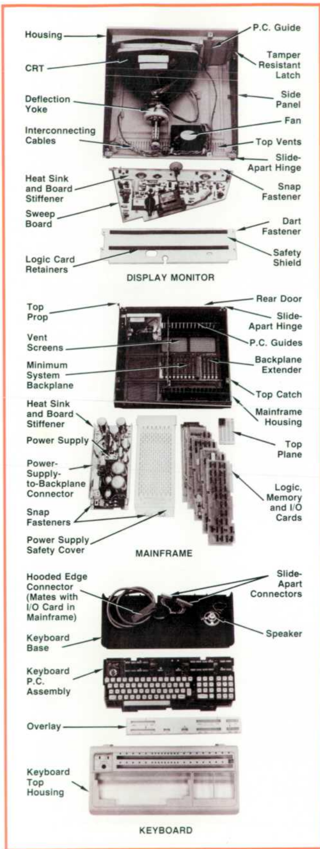
Fig. 1. The 2640A Terminal is designed with pop in/pop-out modularity. The only tool required to replace a module is a key to get inside. Any module can be replaced in two minutes.
