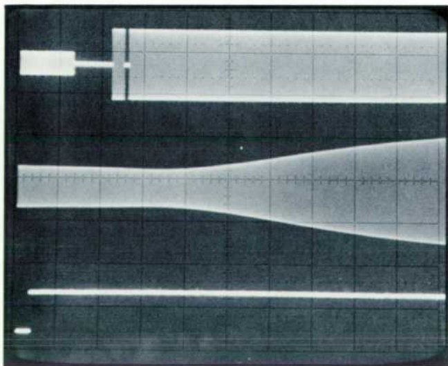
Fig. 2. Oscillogram demonstrates use of the bus analyzer as an oscilloscope trigger (see text). The bottom trace shows the timing of the analyzer's "compare" pulse. The top trace shows the synthesizer output in response to the trigger event and the middle trace shows the output of the filter under test.
