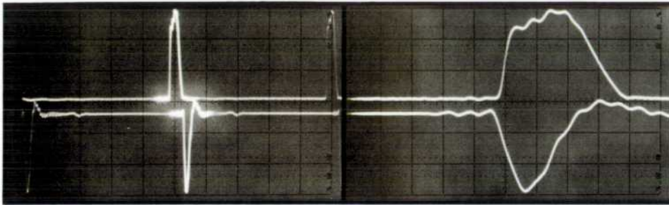
Fig. 7. In the ALTERNATE sweep mode, the oscilloscope measures the time interval between points on two waveforms. Alignment of the two points on the same vertical graticule, in this case the 50% amplitude points as in the photo at right, gives a precise measurement of time interval. (Main sweep: 0.1 \mu s/div; delayed sweep: 10ns/div; time interval: 45.3 ns).
