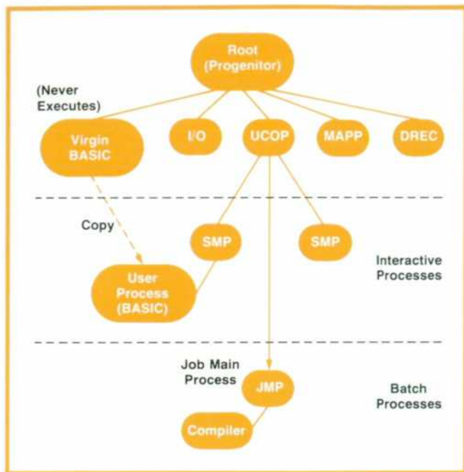
Fig. 3. Since BASIC is invoked so often in MPET, it is permanently linked into the operating system. A virgin BASIC process, created when the first user requests BASIC, is simply copied for subsequent requests.
