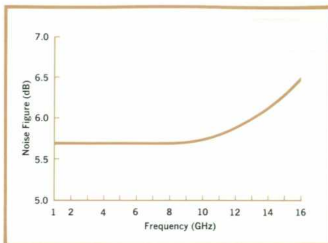
Fig. 6. Noise figure of HP type 5082-2709 diode as a function of frequency.
