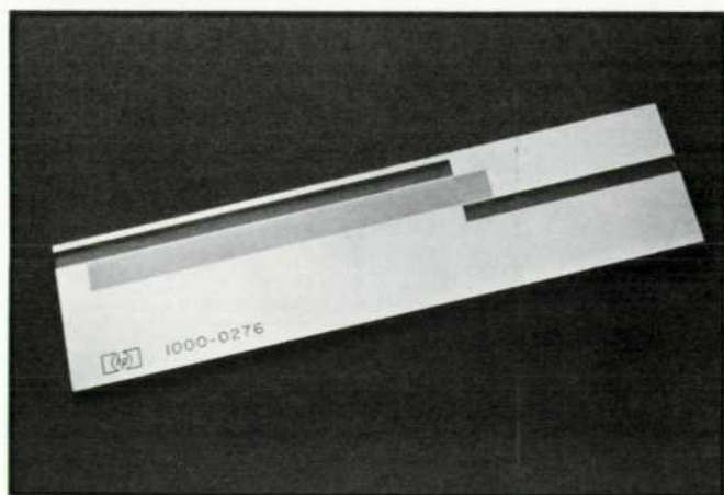
Fig. 1. Encoder plate has 506 line edges that must be accurate within \pm 130 \mu in. The measuring system that checks the plates must be accurate within \pm 10 \mu in.
