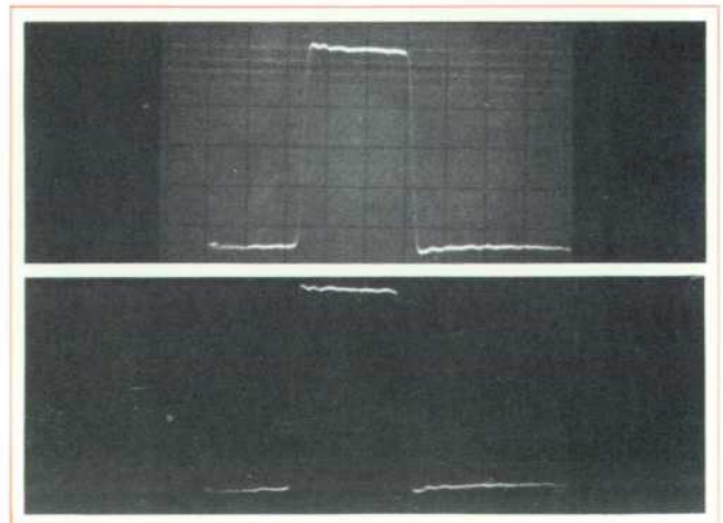
Fig. 2. Trace writing speed is increased by film and phosphor 'fogginess' (upper trace) over speed obtained without fogginess (lower trace), as shown by leading and trailing edges of fast pulse ( t_r = 1.5 ns). Internal flood gun in Model 183A Oscilloscope fogs film and phosphor automatically in synchronism with horizontal sweep.
