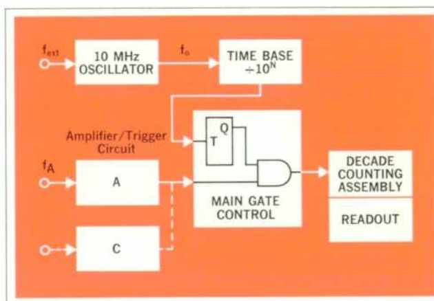
Fig. 3. Frequency measurements can be made using either channel A or channel C. Ratio measurements are made by substituting an external oscillator for the internal clock.
