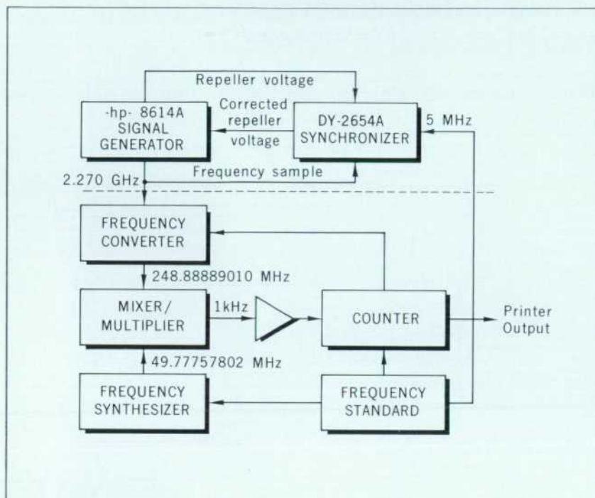
Fig. 2. Instruments above dotted line comprise highly stable microwave source for evaluating stability measurement system shown below dotted line.
