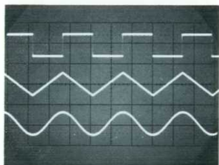
Fig. 6. Multiple exposure oscillogram shows high quality of waveforms produced by new Function Generator. Sine wave distortion is less than 1% from 0.01 Hz to 10 kHz and no more than 3% up to 100 kHz. Square wave rise and fall times are better than 0.25 \mu\text{s} with less than 5% overshoot and 1% sag. Triangular waveform is linear within 1% from 0.01 Hz to 50 kHz and within 2% to 100 kHz. Any two waveforms are available simultaneously. Sync pulse, coincident with triangular and sine wave crests, is available from rear-panel connector.
