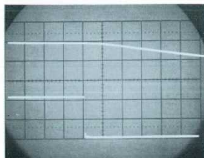
Fig. 9. Oscilloscope shows that output waveform (upper trace) responds to change in frequency control voltage (lower trace) within 0.5 \mu s. Sweep speed here is 1 cm/0.5 \mu sec. Upper waveform is sine wave output of Function Generator, changing from 10 kHz to 100 kHz.
