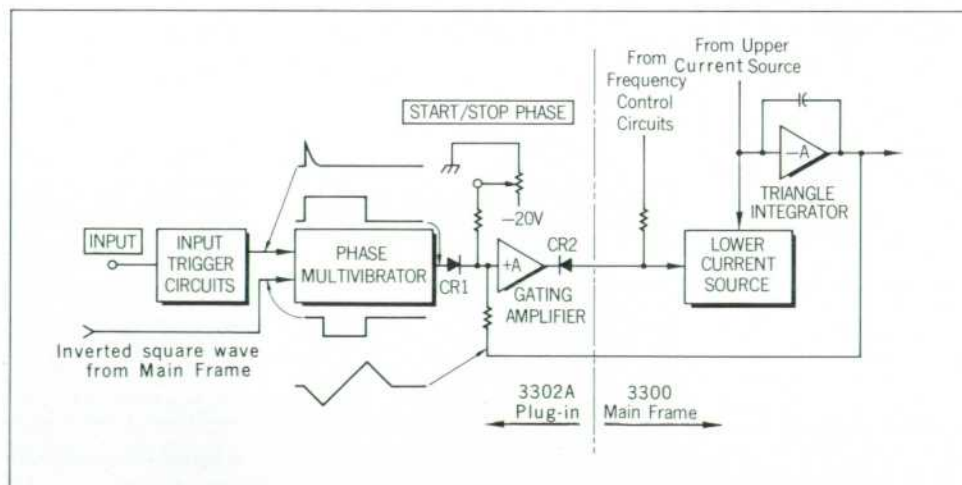
Fig. 2. Block diagram of Trigger/Phase-Lock Plug-in in 'Single' or 'Multiple' modes of operation. (Note: triangular waveform shown here is inverted by output amplifiers before arriving at output terminals.)
