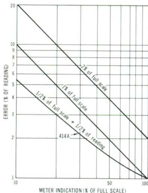
Fig. 1. Accuracy of analog meters as a function of meter deflection. When meter deflection is less than 100% of full scale, -hp- Model 414A Autovoltmeter specification of \pm 1/2\% of full scale \pm 1/2\% of reading is more accurate than 1% of full scale specification. Improvement over 2% specification is correspondingly greater.
