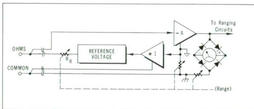
Fig. 5. Block diagram of Autovoltmeter input circuits when switched to ohmmeter mode. Plus-1 amplifier bootstraps Reference Voltage Supply to maintain constant voltage drop across series resistor R_R . Ohmmeter cables are arranged for "4-terminal" resistance measurement.
