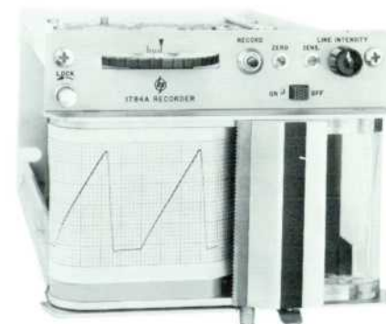
Fig. 2. -hp- Model 1784A Recorder Plug-In. Instrument makes permanent records of recurrent waveforms displayed on scope crt in a few seconds at a cost of about 1½ cents each.
