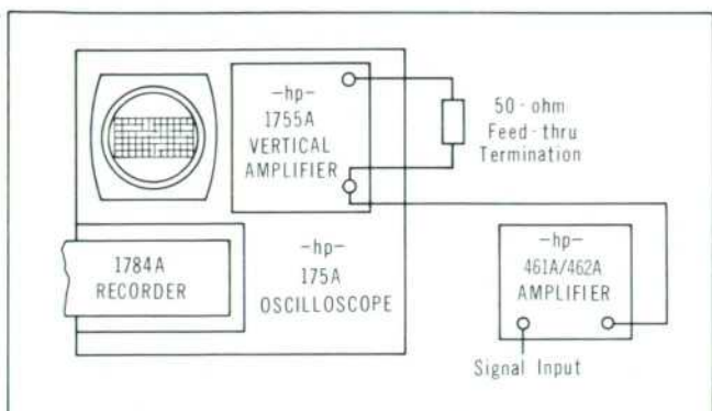
Fig. 3. Instrumentation setup for recording pulses as small as a few microvolts. Model 461A or 462A Amplifier each provide up to 40 dB gain at bandwidths well beyond scope range.
