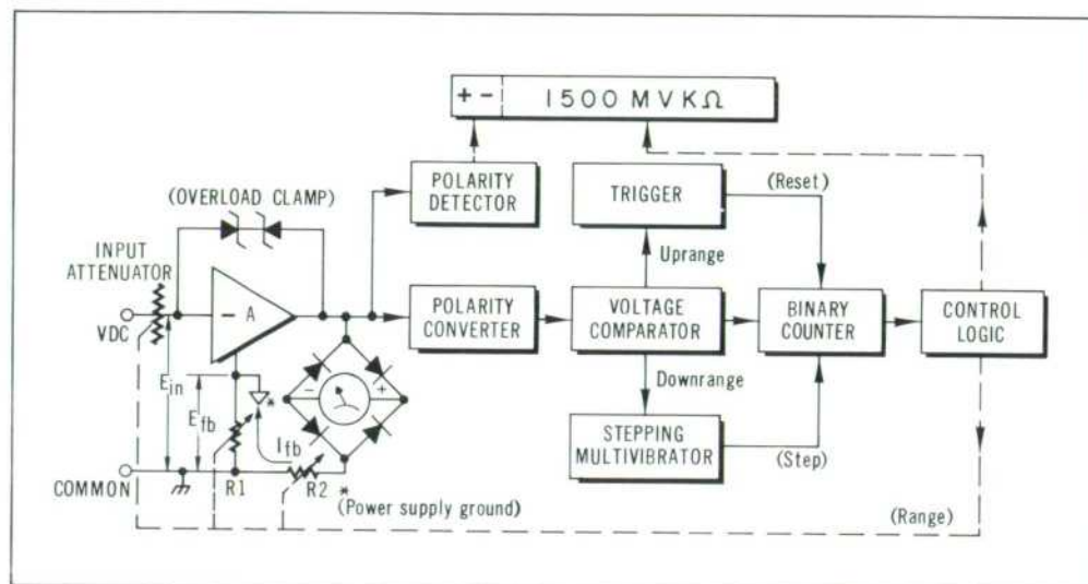
Fig. 4. Block diagram of -hp- Model 414A Autovoltmeter operating in voltmeter mode. Feedback amplifier nulls input voltage E_{in} with voltage E_{fb} across resistor R1 . Range changing is
