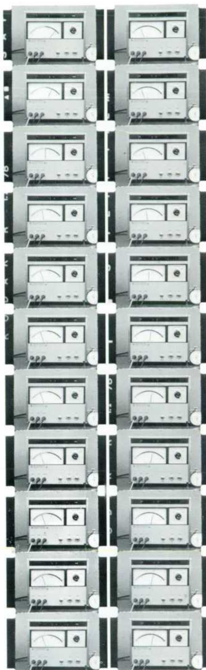
Fig. 3. Speed of response of new Autovoltmeter is shown by film strips photographed at 16 frames per second. In strip at left, input voltage is changed from +14 volts to -15.4 volts following first frame at top of strip. Range change, which requires uprange to 1500V and back down to 50V range, is completed by 3rd frame (polarity change requires no switching other than front panel polarity indicator). Meter pointer stabilizes on new reading by 10th frame. Strip at right shows response speed of meter without range change. Following 2nd frame, voltage is switched from +14V to +29.5V. Meter settles on new value by 9th frame, less than one-half second following voltage change.
