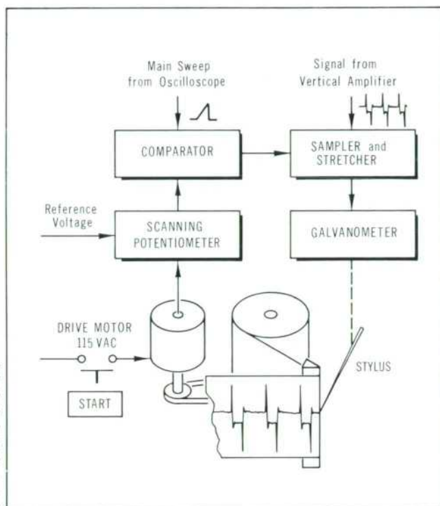
Fig. 3. Instrumentation setup for recording pulses as small as a few microvolts. Model 461A or 462A Amplifier each provide up to 40 dB gain at bandwidths well beyond scope range.
