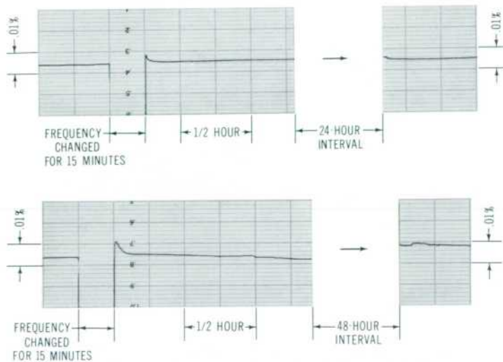
Fig. 9. Repeatability and stability curves similar to Fig. 2 measured on new oscillator at operating frequencies of 10 kc (upper) and 1 megacycle (lower). Note 48-hour rather than 24-hour interval in lower curve.
