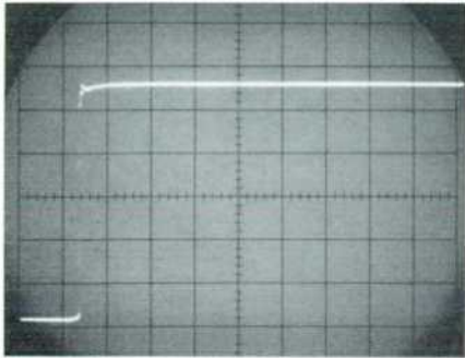
Fig. 2. Oscillogram taken at relatively slow sweep speed of 10 nsec/cm to show flat top of voltage step from -hp- 213B Pulse Generator. Output can be positive or negative. Oscillograms taken on -hp- 185B Sampling Oscilloscope.
