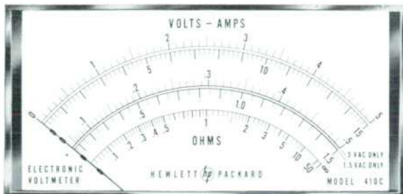
Fig. 6. Detailed view of meter scales. Meter face is calibrated by hp's automatic meter calibrator. Meter movement is of taut-band-suspension type.
