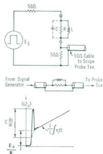
Fig. 8(b) (at right). Explanatory drawing for Fig. 8(a).
