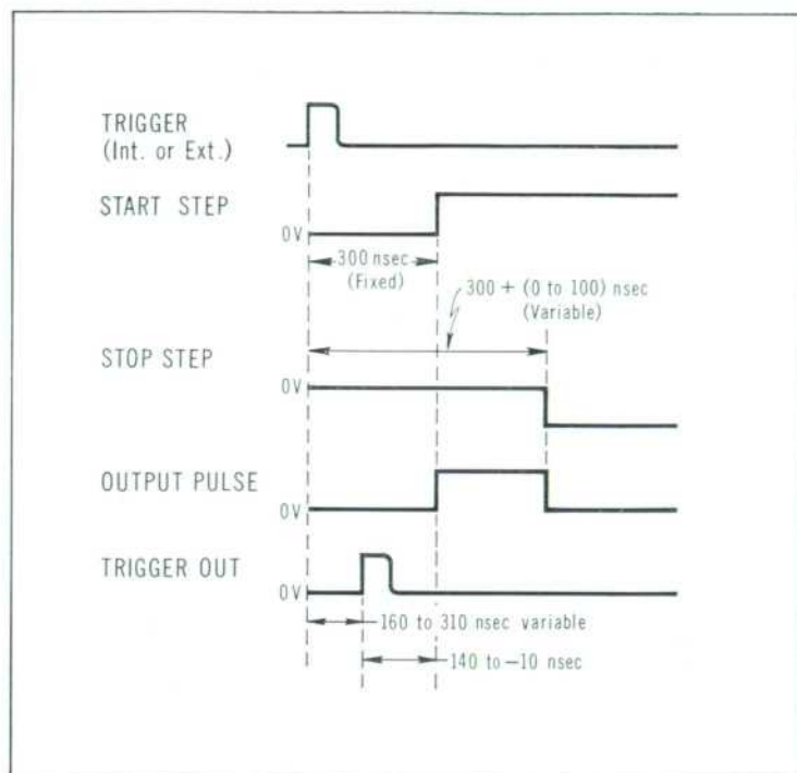
Fig. 8 (at left). Time relations in circuit operation of generator.
