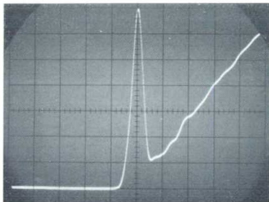
Fig. 1(a) (at left). Oscilloscope showing measurement of small inductance of \frac{1}{4} " leads on 1000-pf capacitor. Vertical scale is calibrated at 1 nano-henry/cm; sweep speed is 2 nsec/cm.
