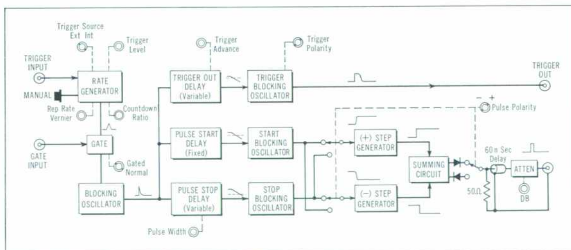
Fig. 7. Basic circuit arrangement of -hp- Model 215A Pulse Generator.
