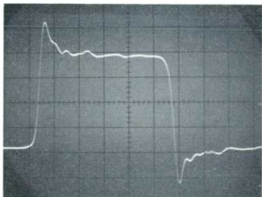
Fig. 9. Oscillogram showing measurement of stray C shunting resistor.
