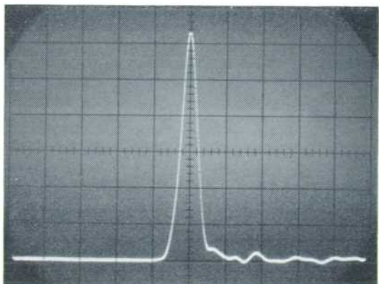
Fig. 2 (at left). Oscilloscope showing how oscilloscope was calibrated for Fig. 1(a) by spike from known length of shorted 50-ohm cable.
