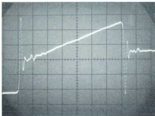
Fig. 8(a) (at left). Oscillograms showing waveforms in measuring small C shunting 1K and 2.2 \mu h R - L combination. Sweep speed is 5 \text{ nsec/cm} .
