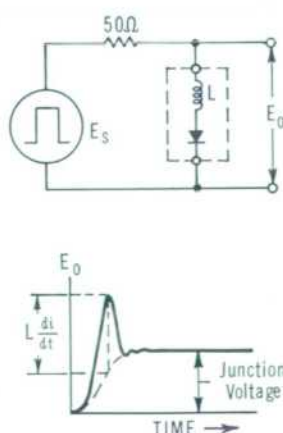
Fig. 6(b). Explanatory drawing for Fig. 6(a).
