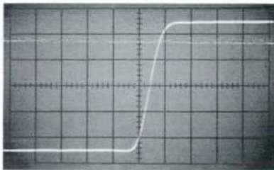
Step response typical of Model 1750A dual-trace plug-in in Model 175A Oscilloscope. Sweep time is 10 nanoseconds/cm.
