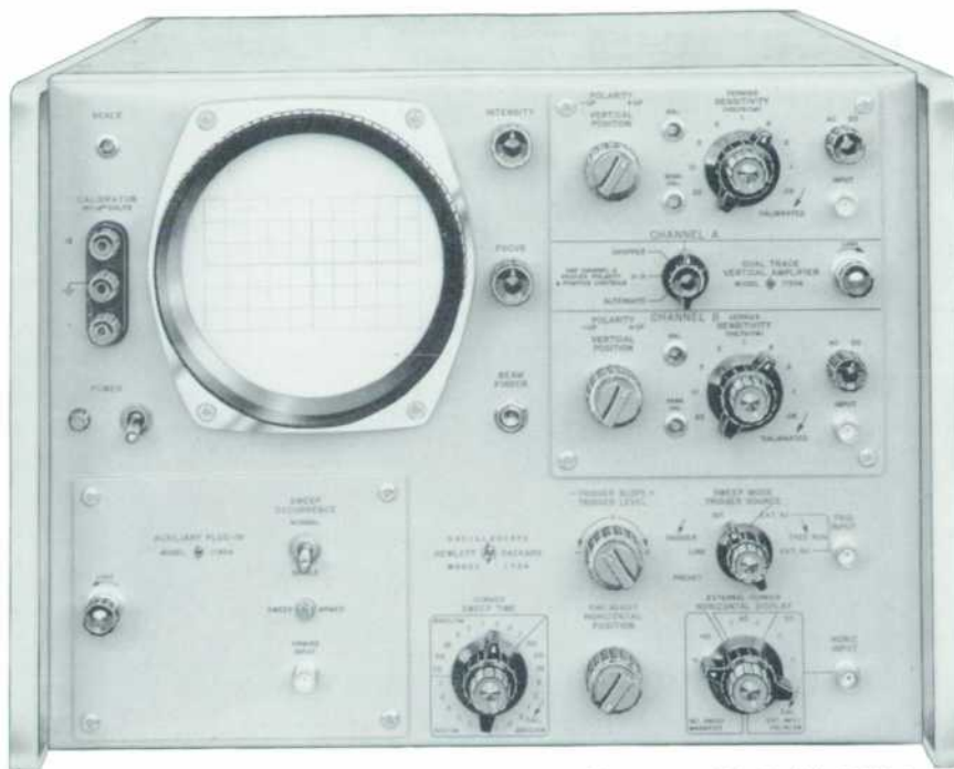
Fig. 6. Panel view of -hp- Model 175A Oscilloscope with Model 1750A dual-trace vertical plug-in and Model 1780A Auxiliary horizontal plug-in. Simplicity of control layout is aided by lack of need for usual astigmatism control.
