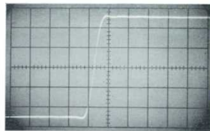
Fig. 5. Oscilloscope of step response of main vertical amplifier. Sweep time is 10 nanoseconds ( 10 \times 10^{-9} sec)/cm. Rise time is less than 6 nanoseconds.
