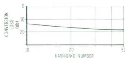
Fig. 5. Typical conversion efficiency of harmonic generator used in new converter unit.
