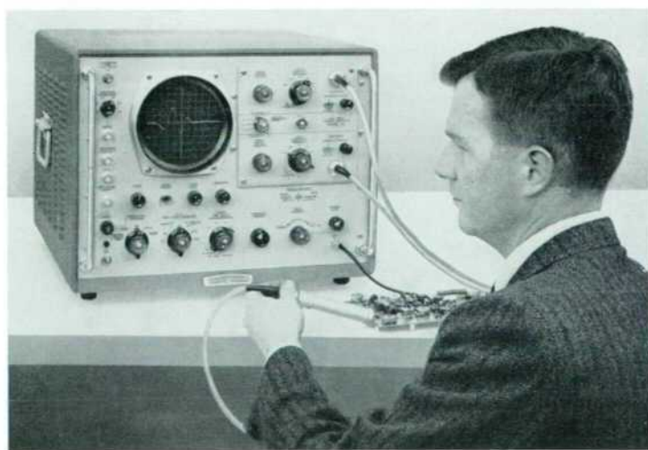
Fig. 1. New -hp- Model 185A/187A Oscilloscope displays signals from 3 millivolts to 2 volts (x10 with adapter) over frequency range up to 500 megacycles. Besides very wide bandwidth and high sensitivity, instrument has several special advantages not found previously in oscilloscopes.
