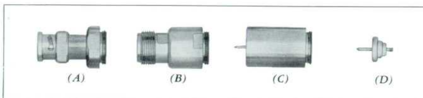
Fig. 17. Adapters available for use with signal probe of Fig. 15.
