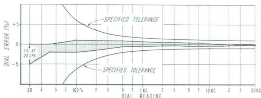
Fig. 8. Extremes of frequency dial error from group of 10 production instruments. Curve shows spread of error among all instruments so that each unit is better than error limits shown. Dial calibration is linear; curve thus also shows that departure from linearity is small.
