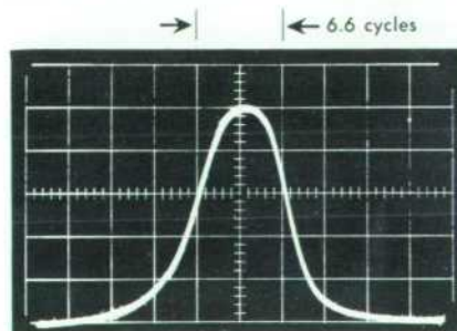
Fig. 2 (above). Dynamic plot of selectivity characteristic of typical 302A analyzer. Three db bandwidth can be seen to be less than 7 cycles. See also Figs. 6 and 7.
