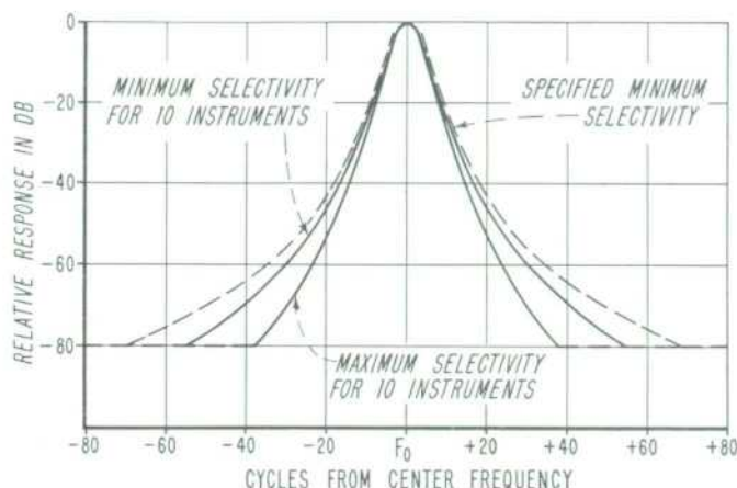
Fig. 7. Typical overall selectivity in the form of maximum and minimum selectivities from group of 10 production instruments.
