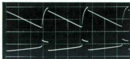
Fig. 2. Oscillogram indicating typical instance where dual-trace oscilloscope permits two-phenomena comparison, here used to check plate and cathode waveforms of phantastron.
