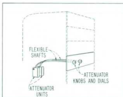
Fig. 2. Single-shaft operation permits attenuators to be mounted in suitable location within racks and operated from panel with flexible shafts or stepping mechanisms.
