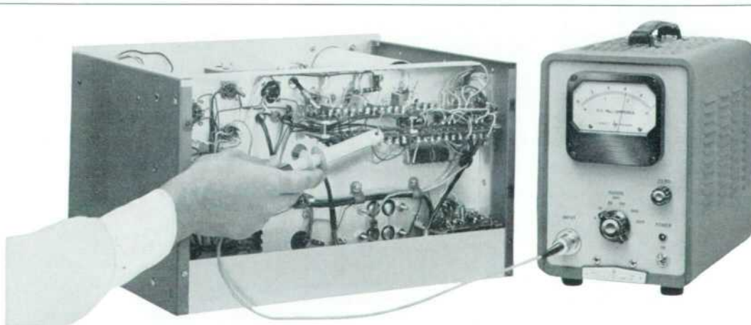
Fig. 1. New -hp- Model 428A Clip-On DC Milliammeter measures dc currents merely by clipping probe around conductor. Current range is from a fraction of a milliamperere to 1 ampere. Probe jaws are operated by flanges on probe body as shown in Fig. 3.
