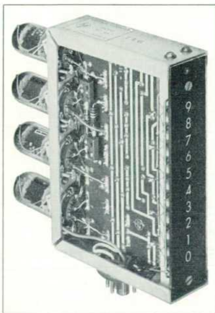
Fig. 1. -hp- 120 kc plug-in decade counter. Design features include etched circuit layout and output staircase.
