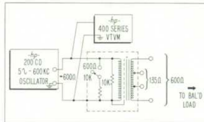
Fig. 5. Connection of 5 kc-600 kc transformer for monitoring signal power.
