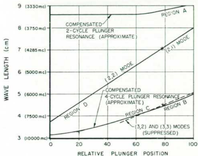
Figure 7. Frequency plot of compensated parallel-plane oscillator.
