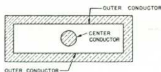
Figure 3. Cross-section of parallel-plane resonator.
