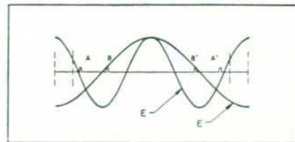
Figure 8. Slots in outer conductors to change natural frequency of peripheral line. Depth of slots is tapered to provide wide-band control.
