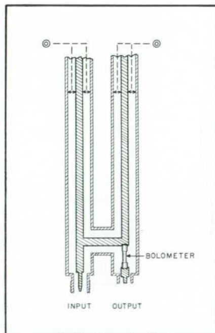
Figure 5. Cross-sectional Drawing of Tunable Bolometer Mount.
