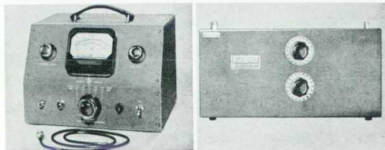
Figure 1. -hp- Model 430A Micro-wave Power Meter. Figure 2. -hp- Model 475B Tunable Bolometer Mount.
