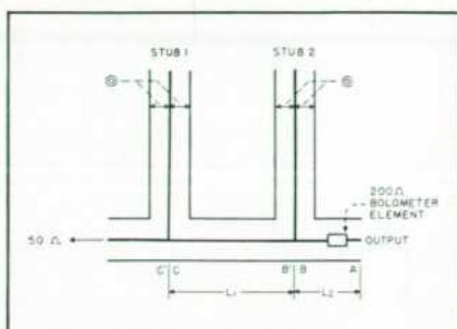
Figure 6. Diagram of Tunable Bolometer Mount.
