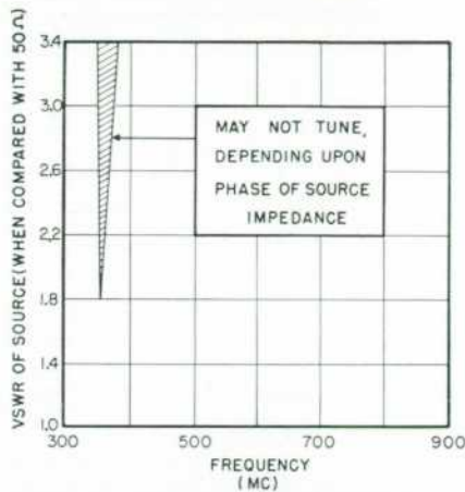
Figure 8. Low Frequency Limits for -hp-475A Tunable Bolometer Mount.
