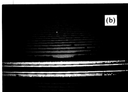
Fig. 10—Observations of single-mode optical fiber preform in (a) monochrome and (b) and (c), colorized form.
