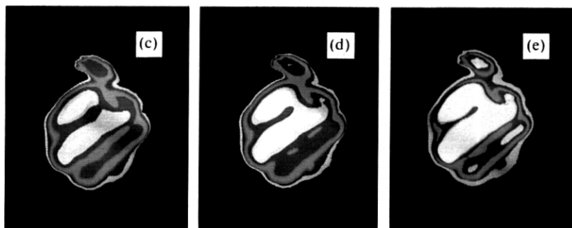
Fig. 6—Near-field light output of poor quality LED observed in black and white and in colorized form as a function of increasing current [(a) through (e)]. Note the changes in the brightest emitting regions shown in white.
