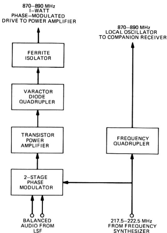
Fig. 17—AMPS cell site transmitter modulator and multiplier.
