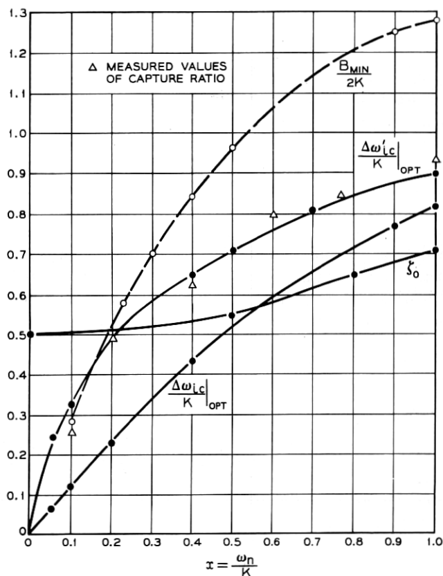
Fig. 7 — Relative noise bandwidth ( B_{\text{min}}/2K ), capture range approximations ( \Delta\omega_{ic}/K ) and (\Delta\omega'_{ic}/K) and damping factor \zeta_0 as a function of (\omega_n/K) for an APLL optimized for minimum noise bandwidth.
