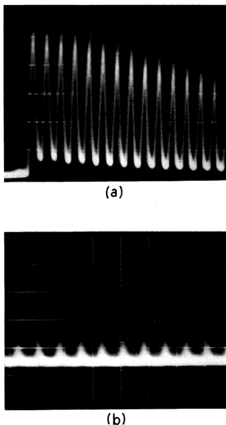
Fig. 4 — Individual pulses: (a) first 13 round trips, (b) round trips number 300 to 310.
