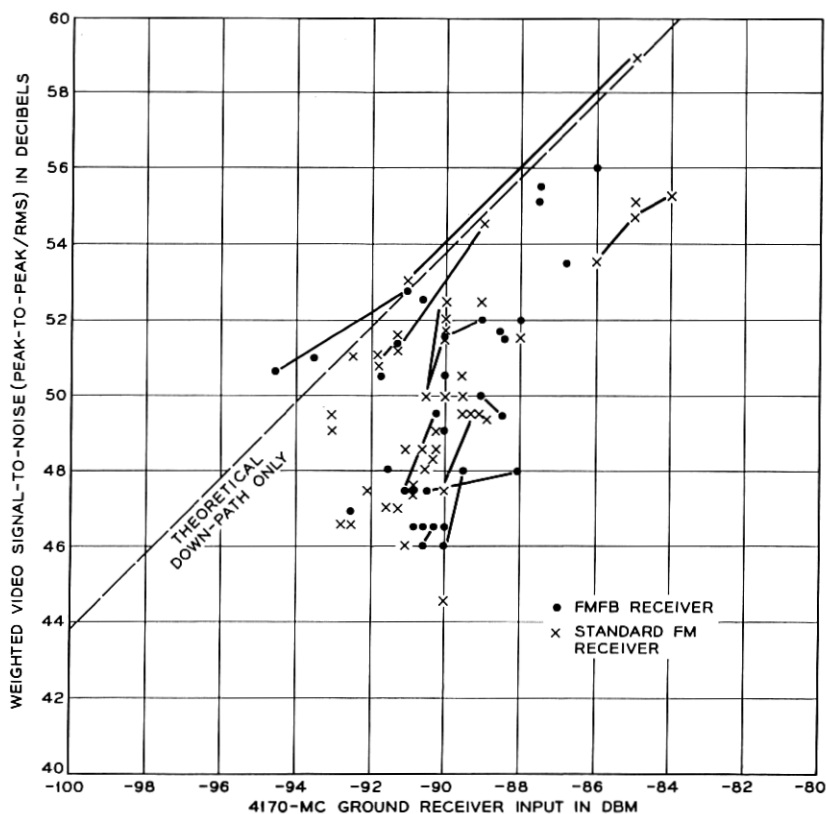
Fig. 24 — Video noise vs received carrier power.
