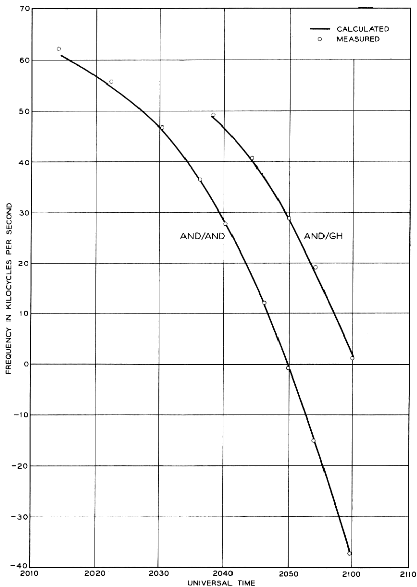
Fig. 52 — Doppler shift of communications carrier; pass 443, Aug. 27, 1962.
