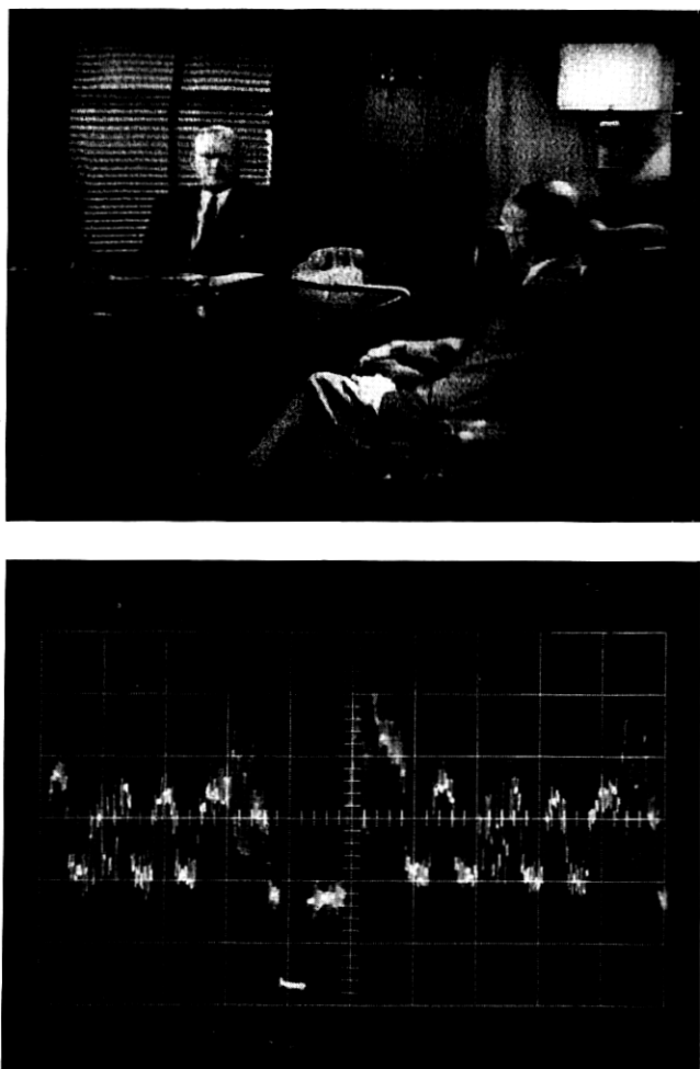
Fig. 43 — Television signal transmitted to France and returned to Andover; pass 142, July 25, 1962. Top: monitor presentation. Bottom: oscilloscope presentation of individual lines.
