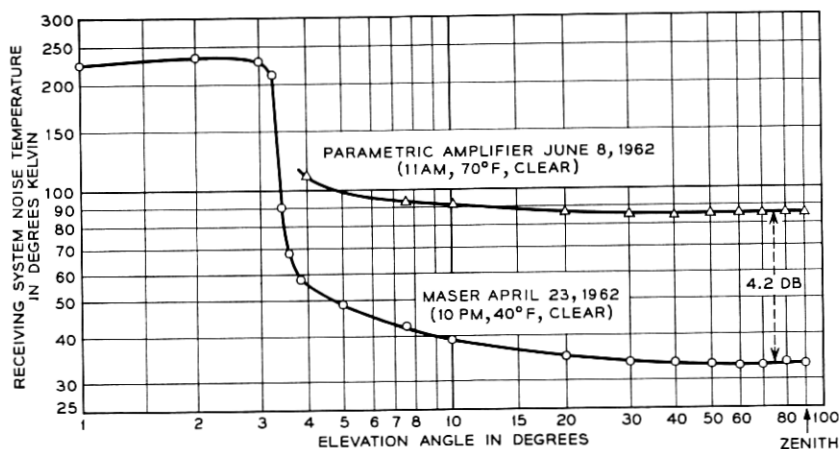
Fig. 15 — Receiving system noise temperature as a function of antenna elevation — clear day data. Azimuth = 142°.
