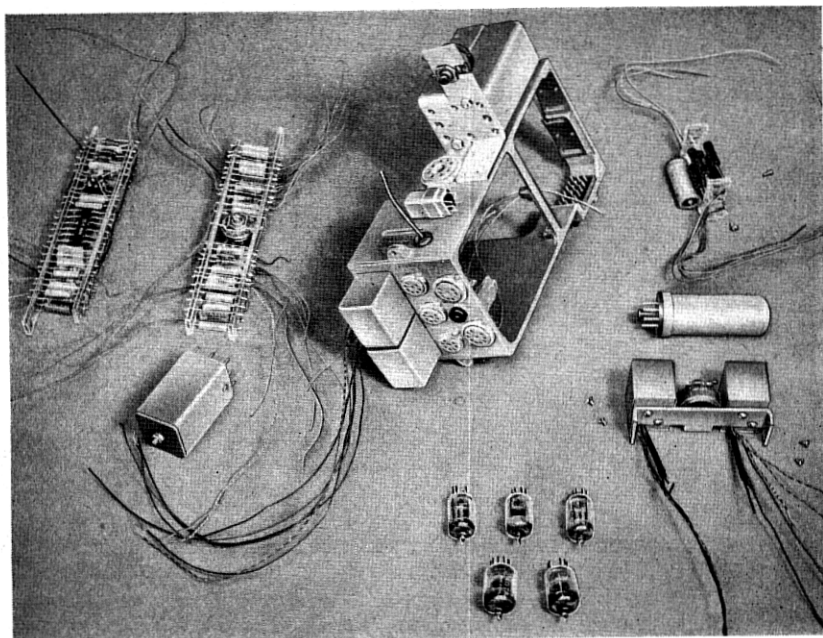
Fig. 18—An exploded view of the expandor and signaling subassembly ready for the final assembly operation. This shows the extent to which prewiring of small assemblies is used.
