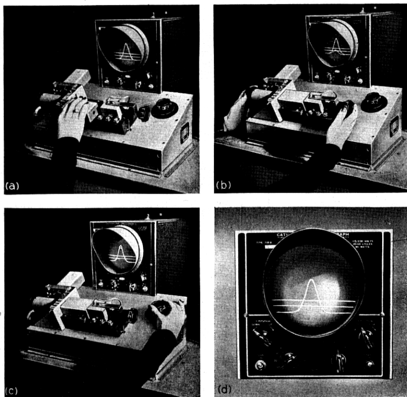
Fig. 9—(a) Operator inserting test filter in jig. Traces appearing on the cathode ray tube are the characteristic of a reference filter and two reference discrimination levels. The lower trace represents transmission in the test path, which circuit has not yet been completed. (b) Unadjusted filter characteristic appears on lower trace. (c) Adjustment completed, mid-band loss level being checked for limits. (d) Close-up of cathode ray tube which shows characteristic of filter under test coinciding with the characteristic of the reference filter.
