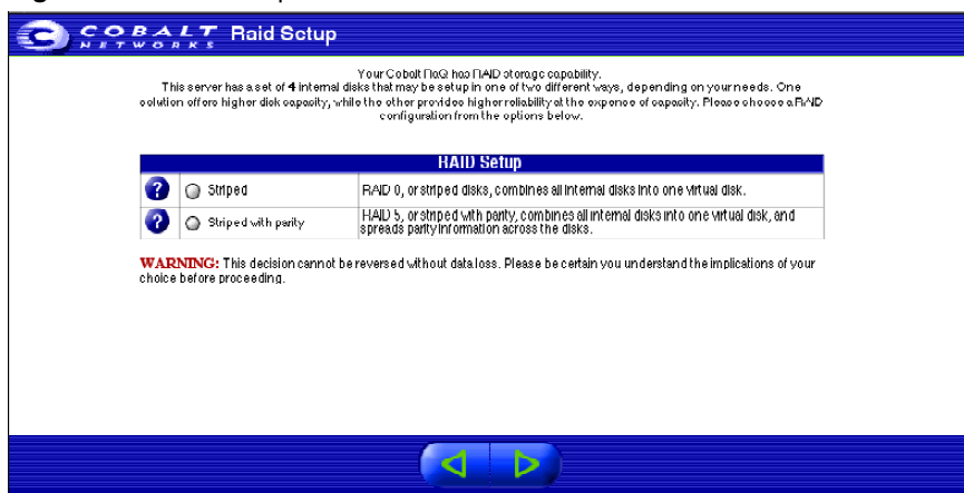
Figure 13. RAID setup
