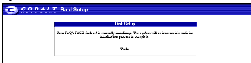
Figure 14. RAID initialization
