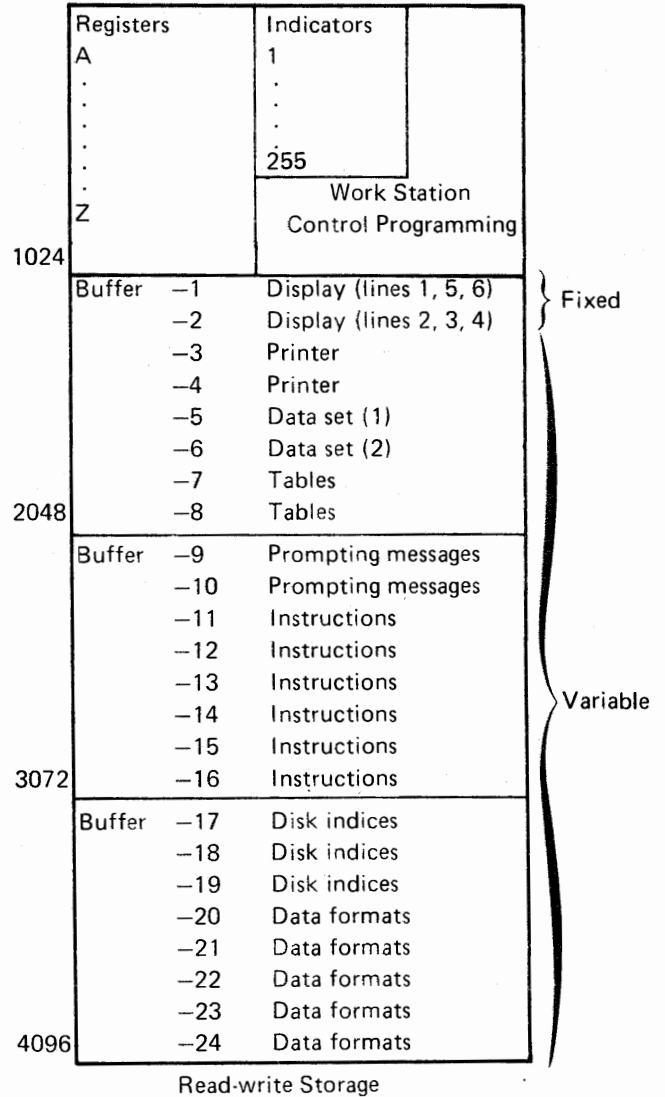
Figure 3. ACL Program Structure
