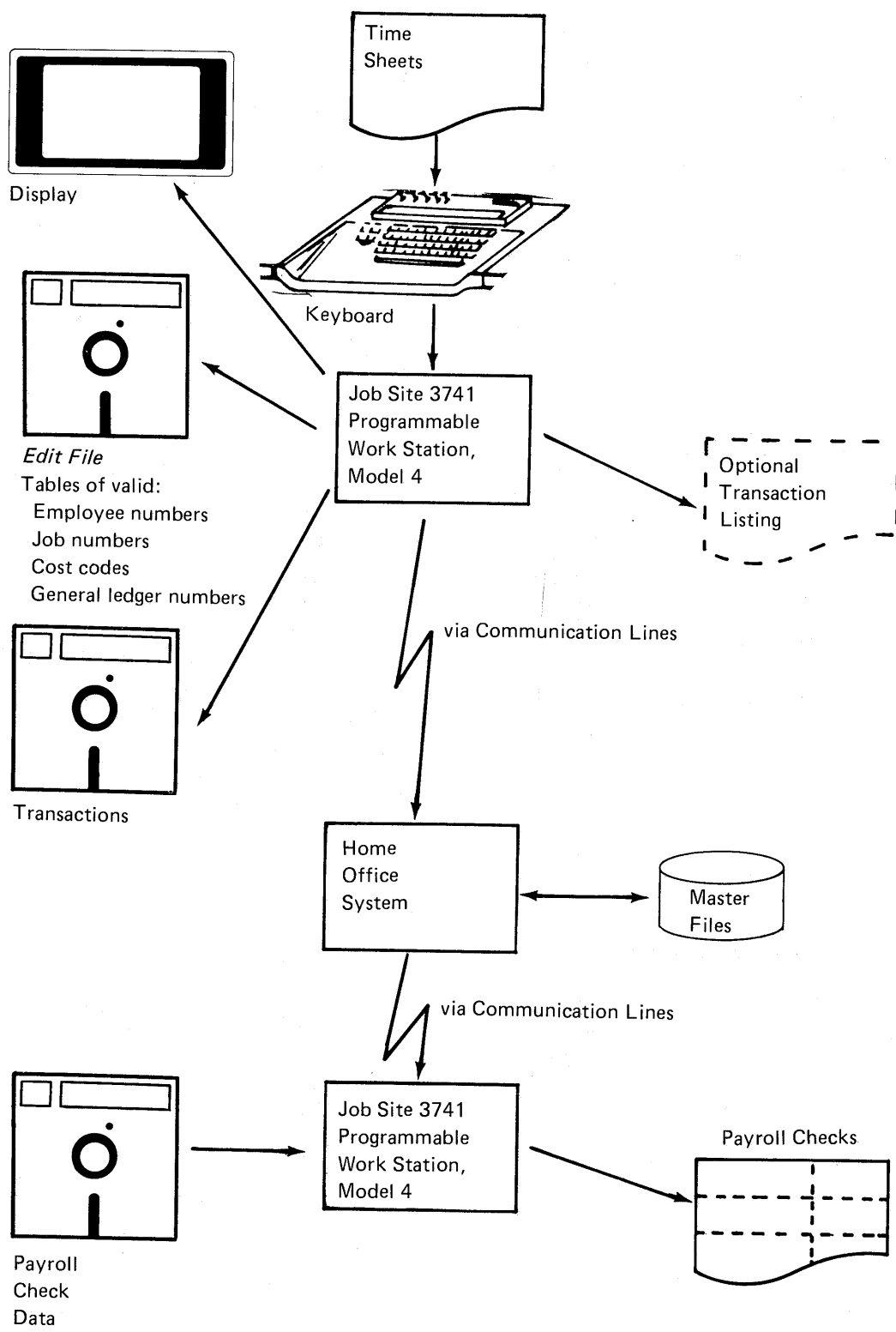
Figure 10. Construction Job Site Reporting – Payroll
