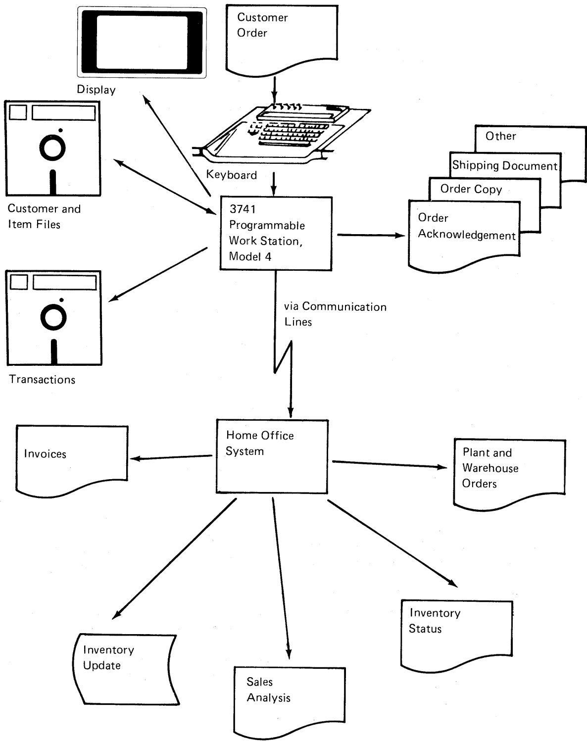
Figure 4. Warehouse Order Entry Data Flow
