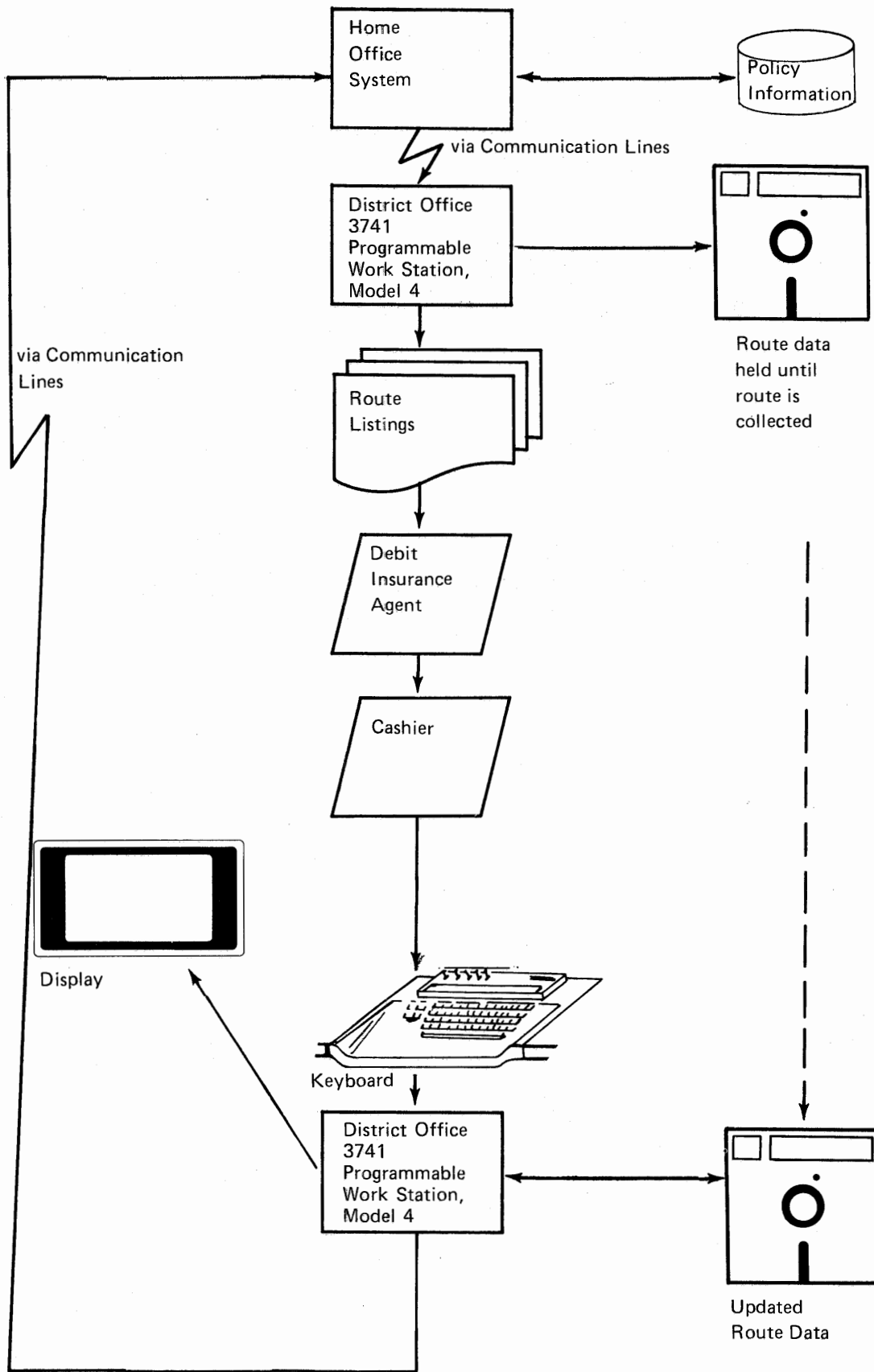
Figure 13. Debit Insurance Data Flow
