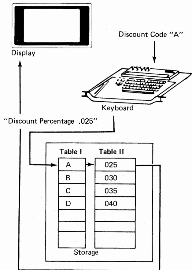
Figure 2. Search Table for Equal Entry – Read from Second Table
