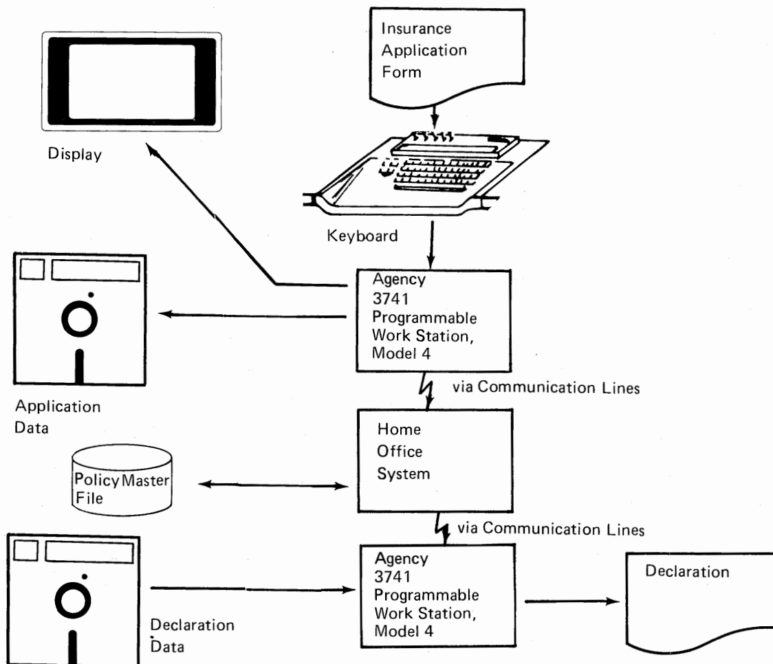
Figure 6. Automotive Insurance New Policy Data Entry
