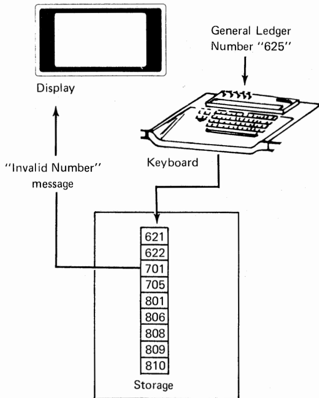
Figure 1. Table Search for Equal Entry
