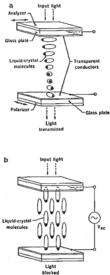
FIGURE VIII Liquid-crystal Display
