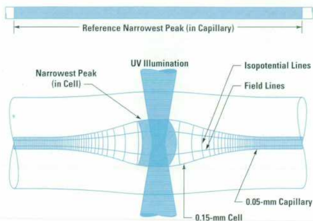
Fig. 4. Electrical field model of the cell.
