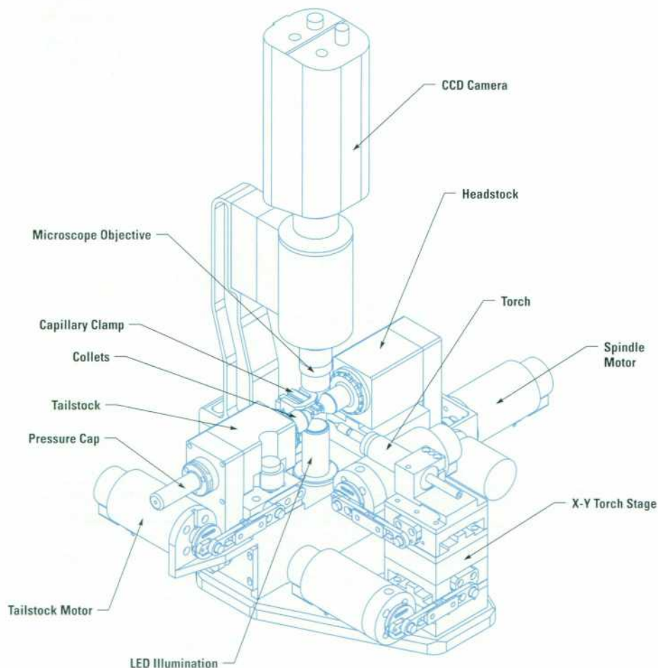
Fig. 6. Schematic drawing of the tabletop-size custom microglass lathe, nicknamed BubbleWorld, which incorporates four servoed axes and machine vision.
