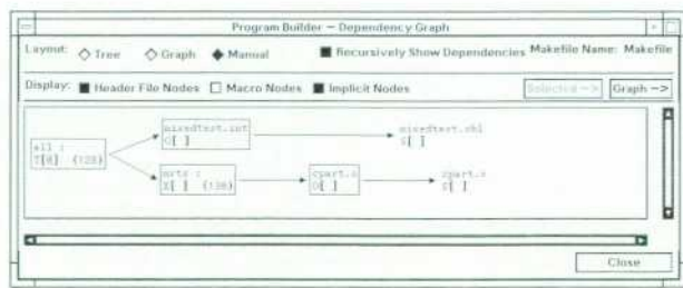
Fig. 13. Dependency graph to verify that the makefile is correctly identifying a mixed-language file.
