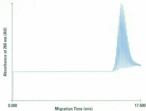
Fig. 5. A CGE separation of oligoadenylic acids. The oligomers range from 40 to 60 units in length.
