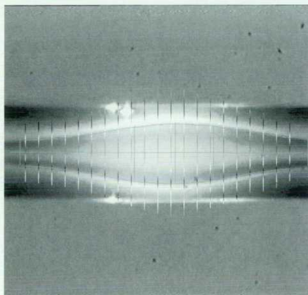
Fig. 10. After blowing is complete, time is less critical and a more complete characterization can be made. The MEASURE operation determines the cell diameter, length, and axial position to an accuracy of 2%.
