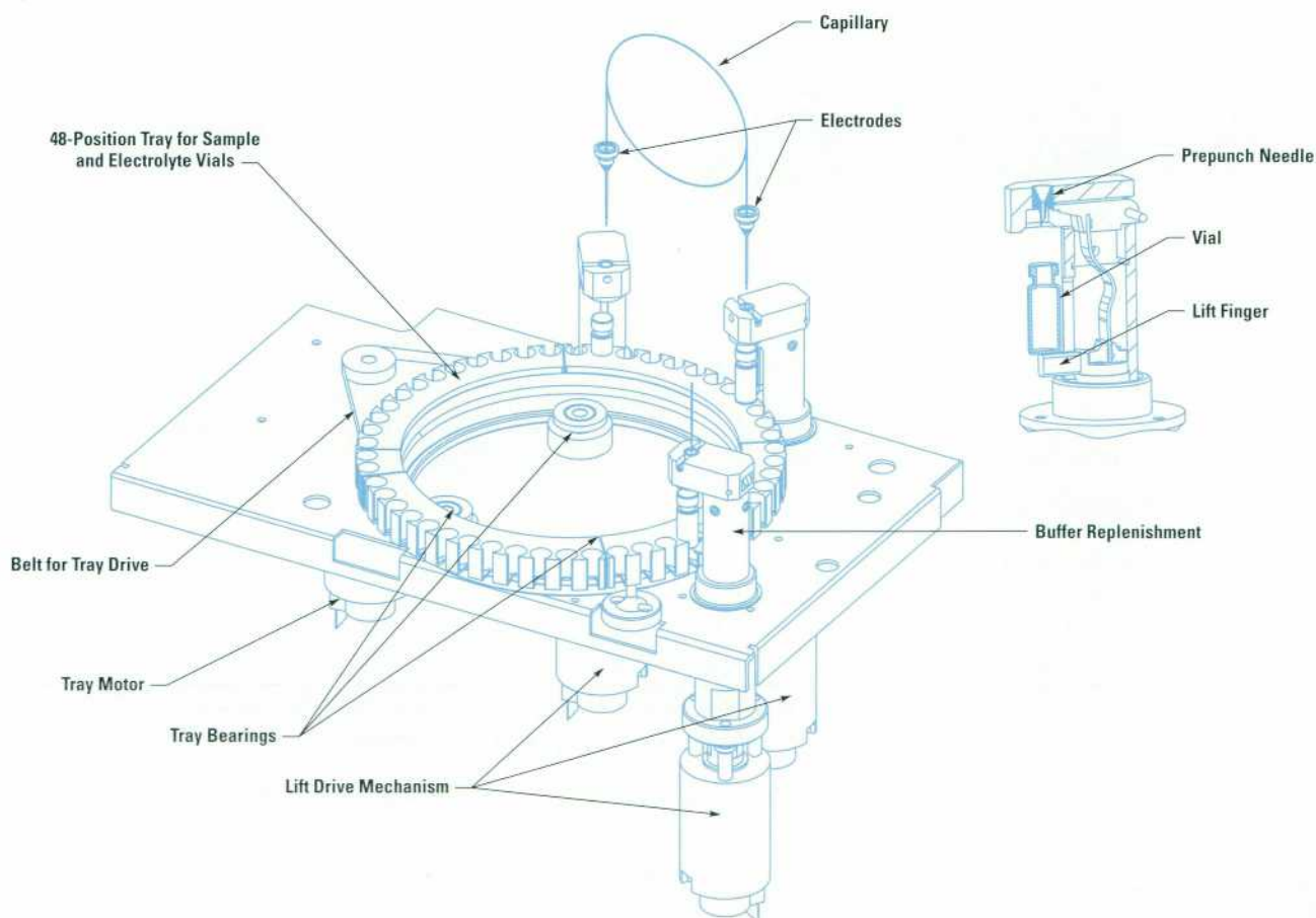
Fig. 8. Liquid handling system.
