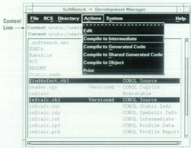
Fig. 3. Selecting several COBOL files for compilation.
