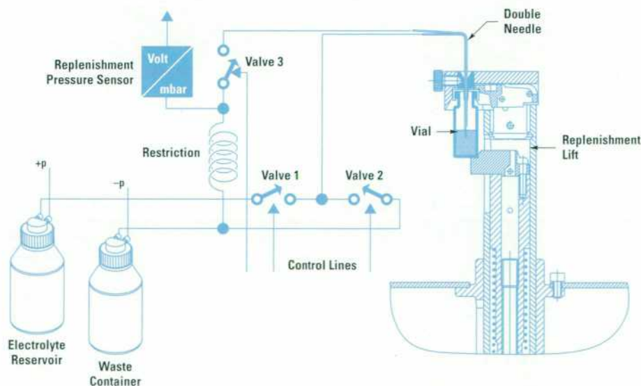
Fig. 4. Replenishment system.
