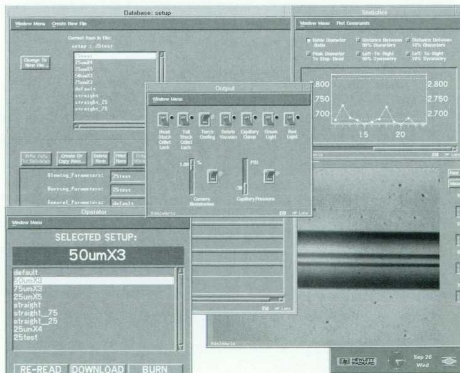
Fig. 7. A custom graphical user interface (GUI) was designed to allow the user to develop, execute, and monitor the manufacturing process easily. There are windows for setting up parameters, collecting statistics, and displaying live video of the forming bubble.
