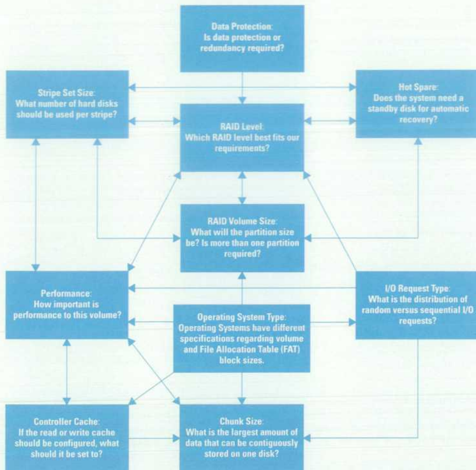
Fig. 6. Dependency relationships between RAID parameters.
