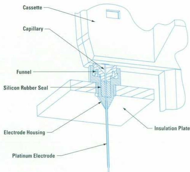
Fig. 3. Electrode details.
