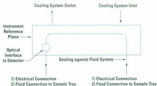
Fig. 3. Capillary interfaces to the instrument infrastructure.
