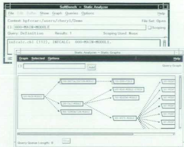
Fig. 8. The SoftBench static analyzer and the static graph showing the structure of the calculation program.
