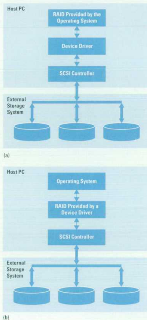
Fig. 4. Software approaches to implementing the RAID technology. (a) Software inside the operating system. (b) Customized software drivers.
