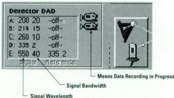
Fig. 9. Detector display.
