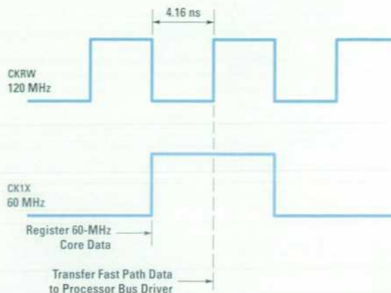
Fig. 3. Fast path timing.
