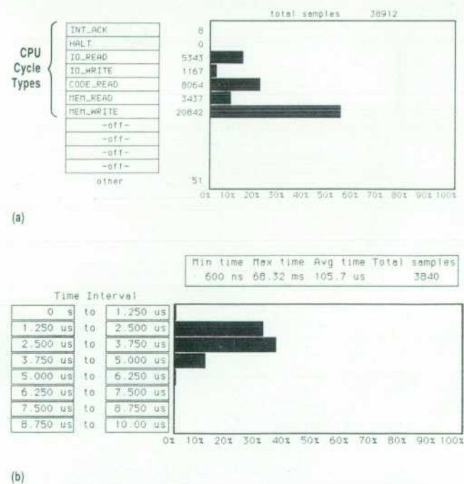
Fig. 3. Sample histograms from an HP 16500 logic analyzer. (a) The occurrence mix of a subset of Intel486 CPU cycle types. (b) Interarrival times of writes to video memory.
