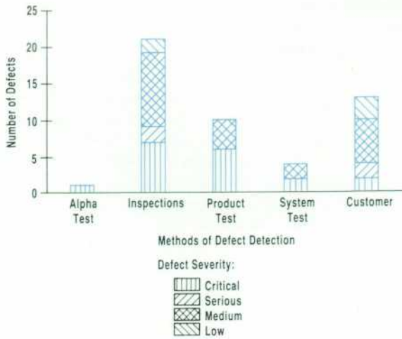
Fig. 5. Defects categorized by severity and method of detection.
